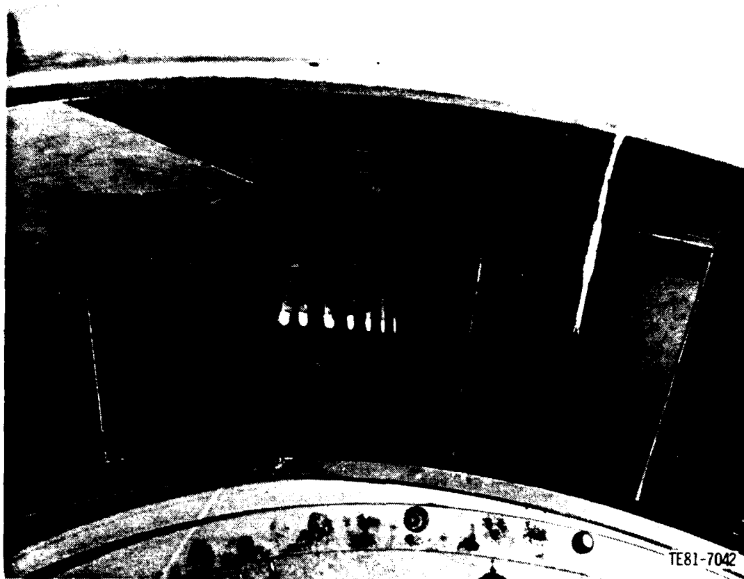
Figure 7. View of typical hot-wire installation in low speed compressor vane row.
