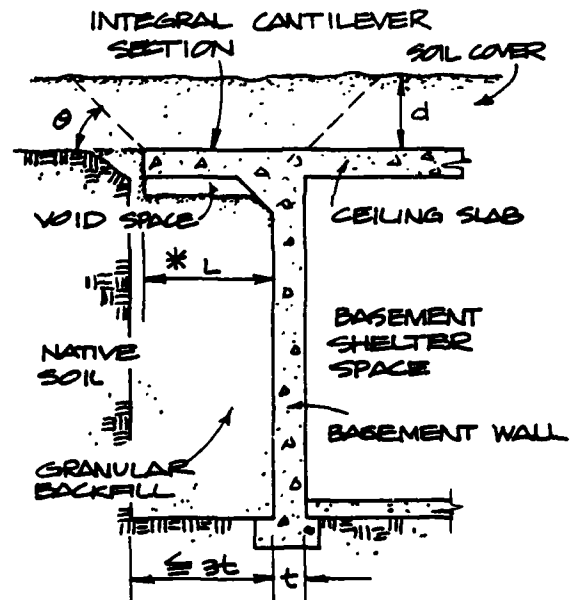
* L TO BE DETERMINED BASED ON EXPECTED TYPE OF SOIL COVER AND DEPTH d. d. Use of Integral Cantilever
