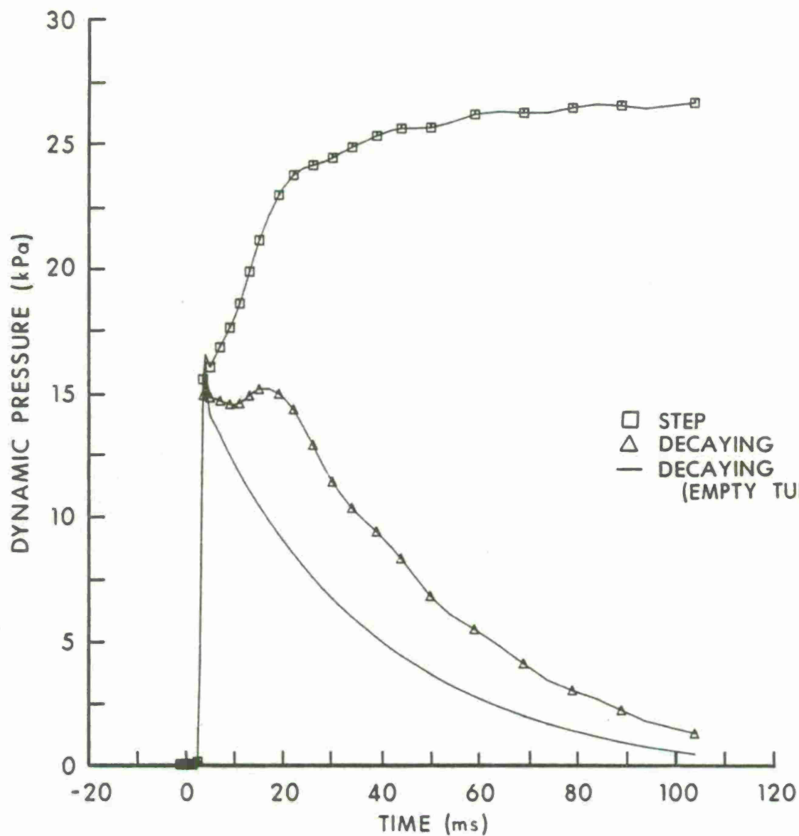
Figure 19. Average dynamic pressure between the cylindrical target and the outer-radial boundary for 68.9 kPa shocks with 20 percent blockage.
