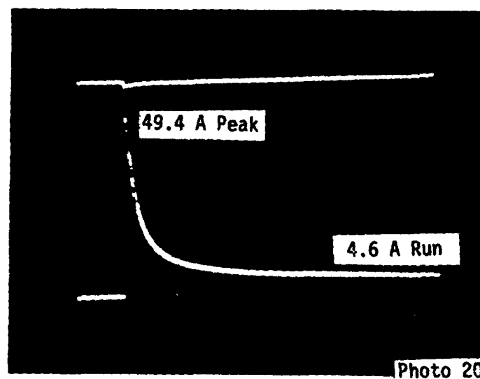
#2 DC Blower, 41.8^{\circ} F, 28 Vdc Open Flow
