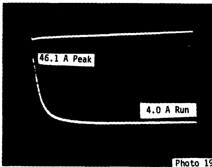
#1 DC Blower, -38.2^{\circ} F, 28 Vdc Open Flow
