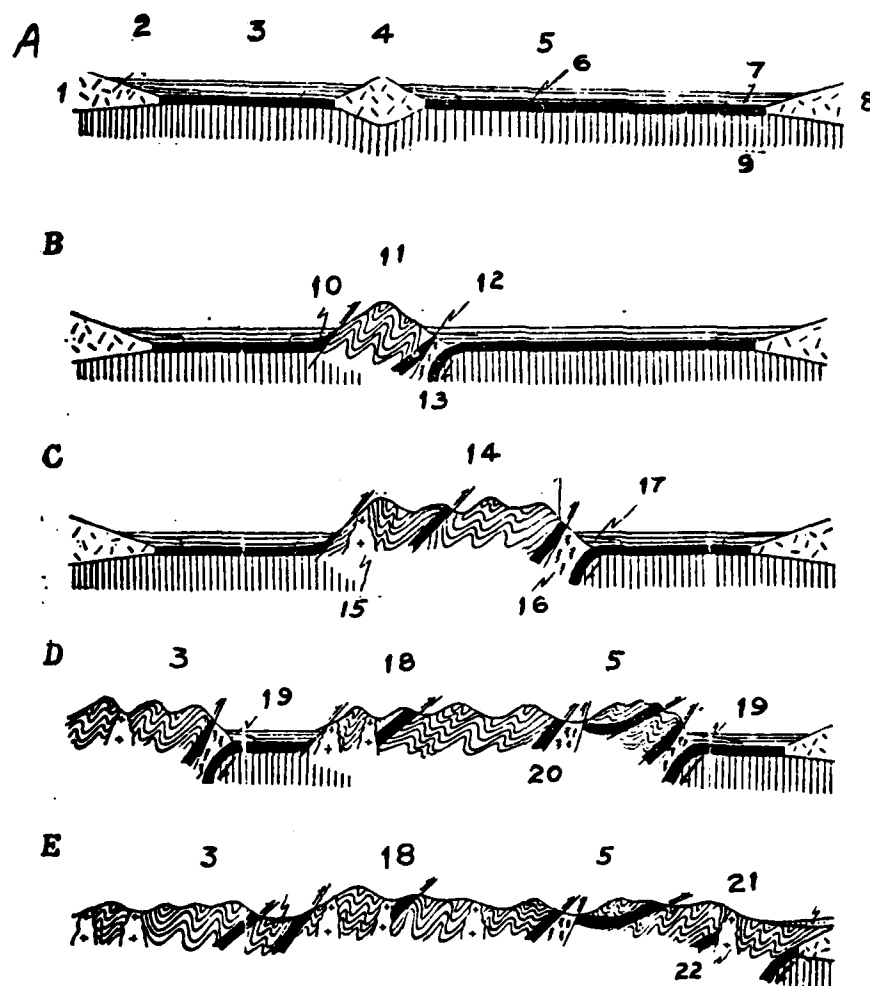
Fig. 5. Tectonic evolution of Chilen (western section). (10) A. The Sinian paleogeography and the formation of its oceanic crust. B. During the early Caledonian movement, the first episode: The oceanic plate broke at the northern border of the Middle Chilen Island Arc. C. The second episode: the oceanic crust twice plunged southwards along the northern border of the Middle Chilen upwarping zone. Along the deep ocean trench, middle and upper ordovician flysch deposits formed. D. Third episode: The oceanic plates plunged for the third time southwards along the northern borders of the Southern and the Northern Chiliens separately, and the Silurium strata were formed along these two lines. E. The fourth episode involved the collision of the Alashan block against the Eulublunk uplift and its epicontinental mountains, and formed Devonian Mullite deposits at the northern border of the Northern Chilen range.
