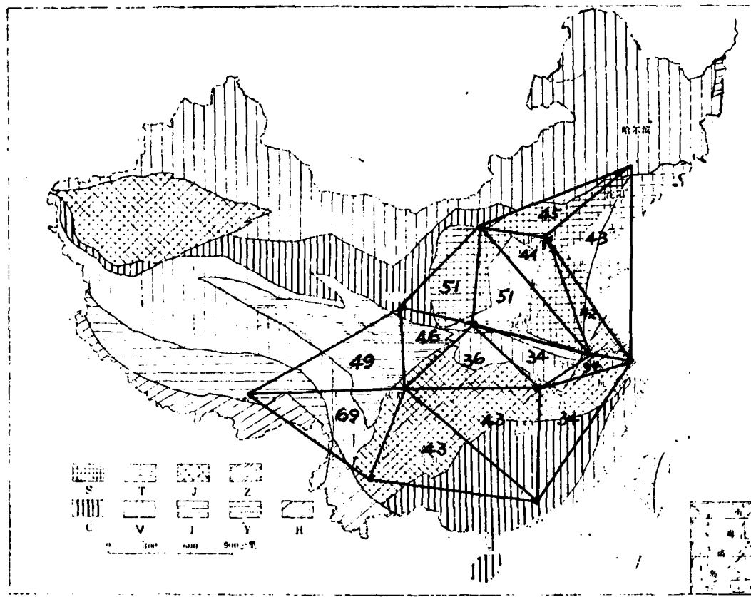
Fig.20 Depth of Moho surface calculated from surface wave (shown by the number in triangles, in km) (17)
