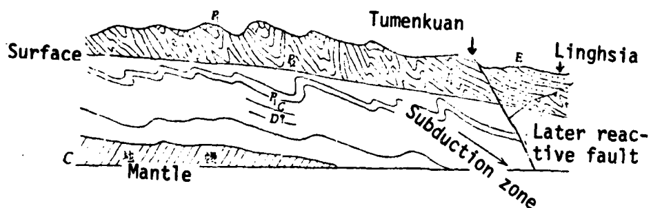
Fig. 10. Constructed profile of the production and development of Mélange at the northern part of West Chilien.
