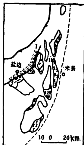
Fig. 14. Metamorphism zone in pairs at Yanbian-Miyi. (7)
