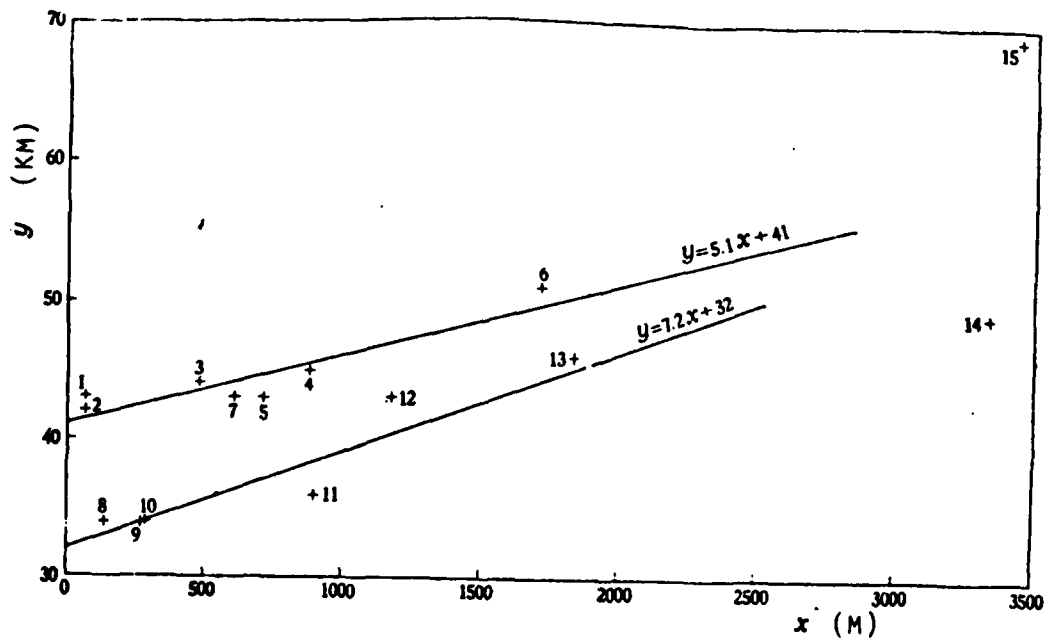
Fig.21 Moho's surface depth-altitude. (17)
