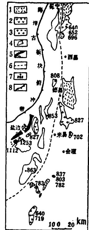
Fig. 12. Distribution of Precambrian intrusives and extrusives at Kangtien Kern. (2)
