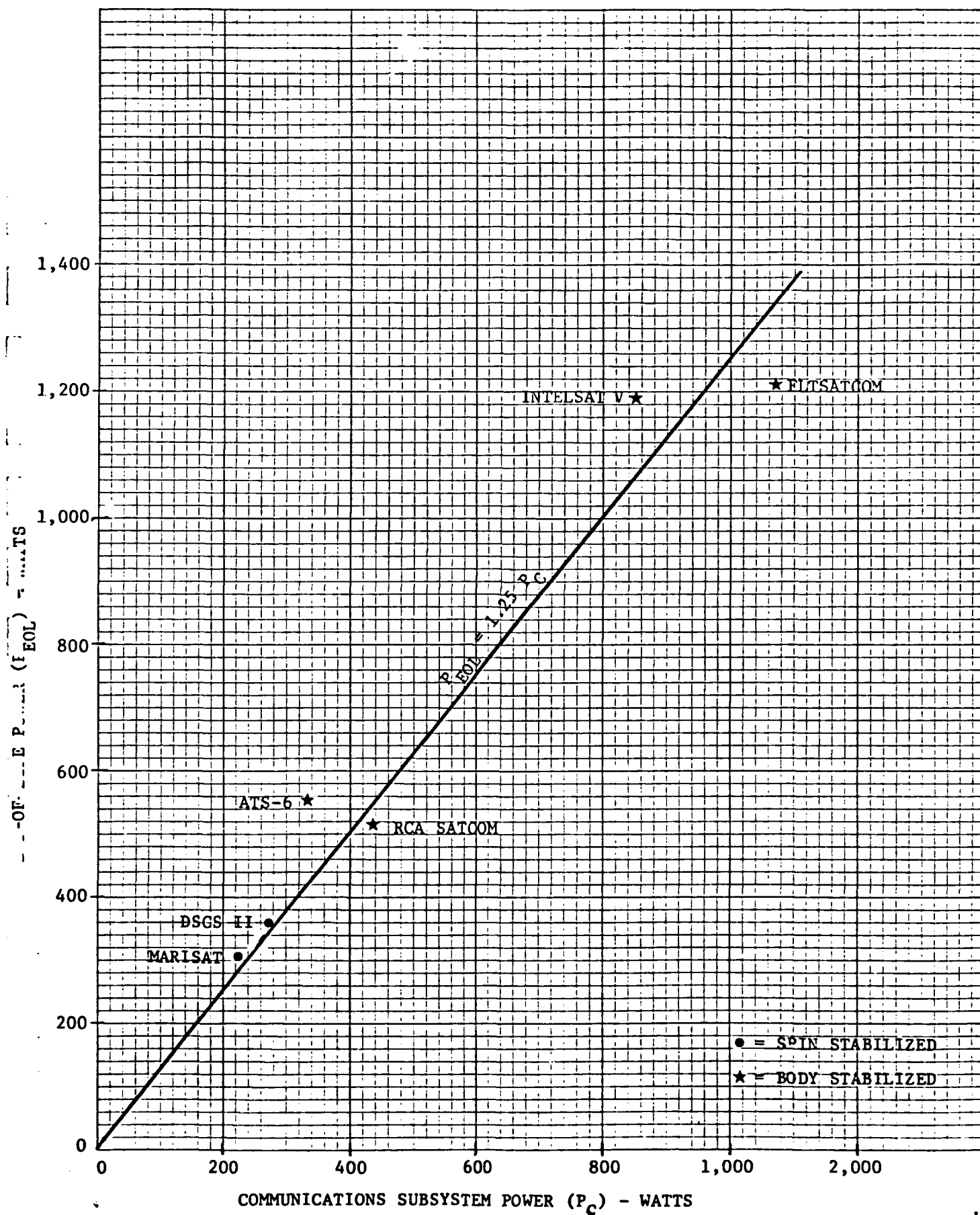
FIGURE III-1. END-OF-LIFE POWER
