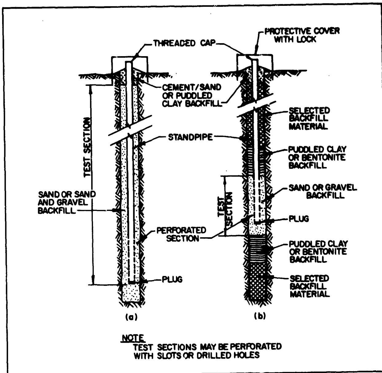
FIGURE 7 Open Standpipe Piezometers
