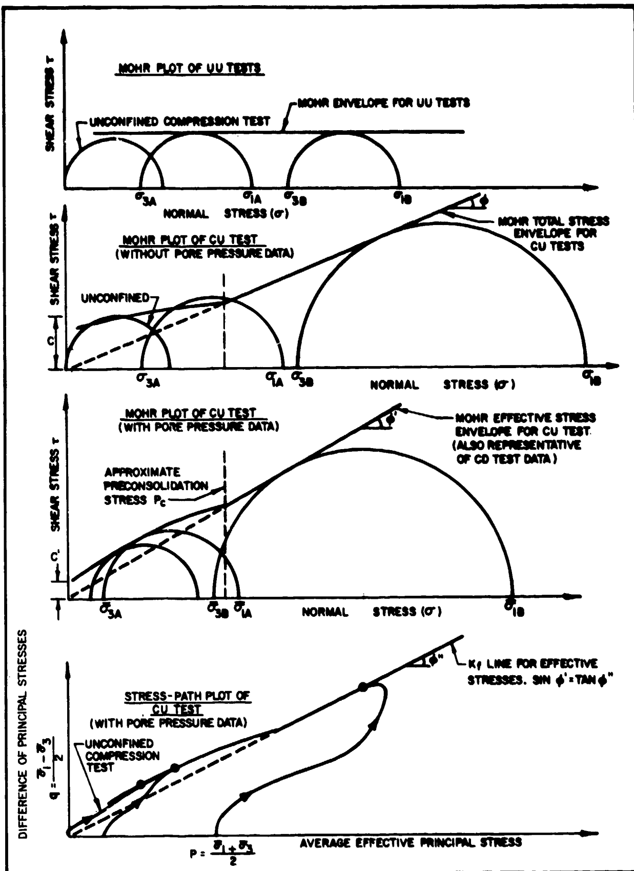
FIGURE 6 Triaxial Shear Test Relationships 7.1-147
