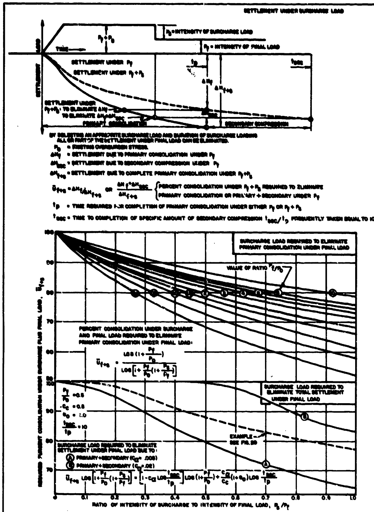
FIGURE 17 Surcharge Load Required to Eliminate Settlement Under Final Load
