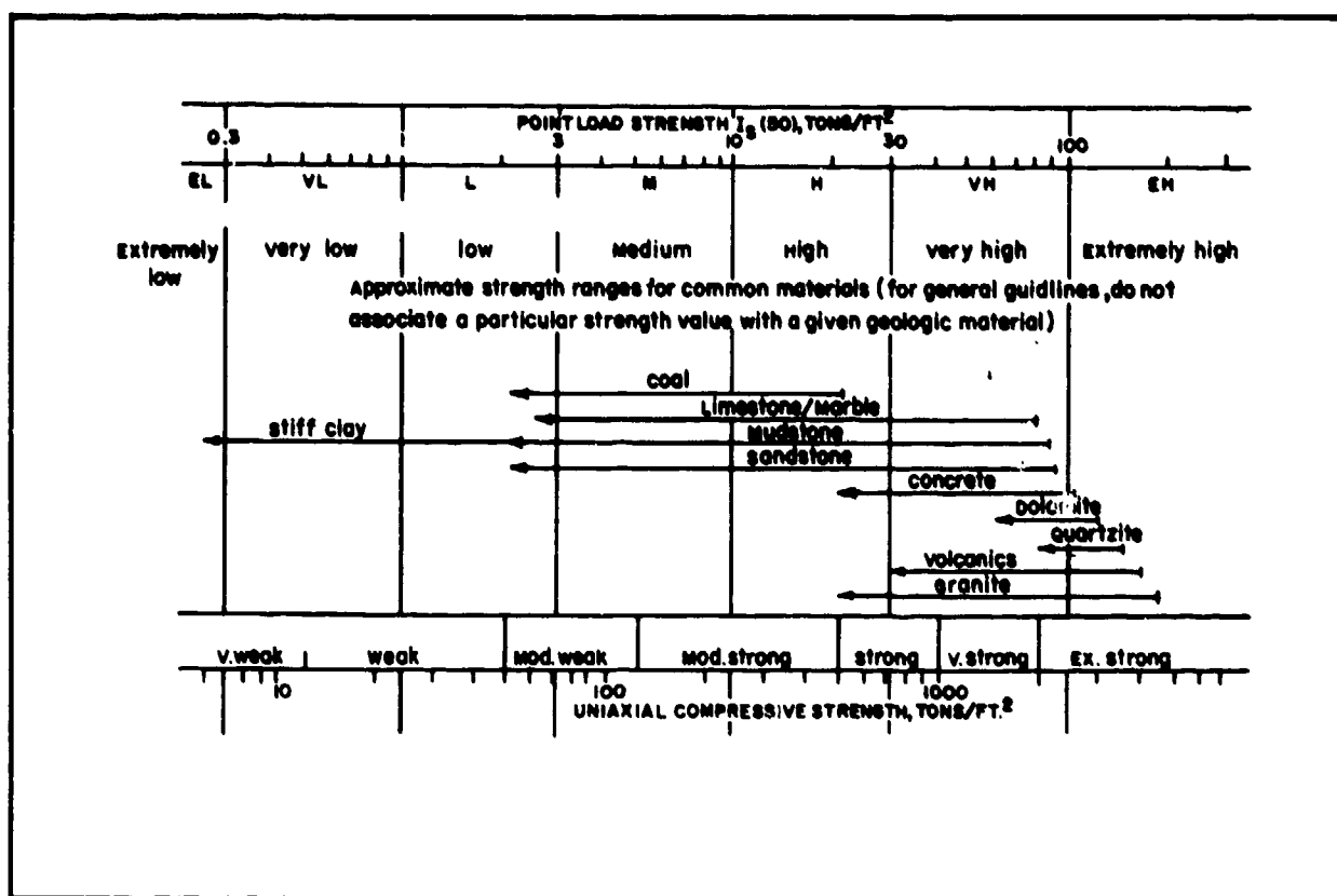
FIGURE 3 Strength Classification
