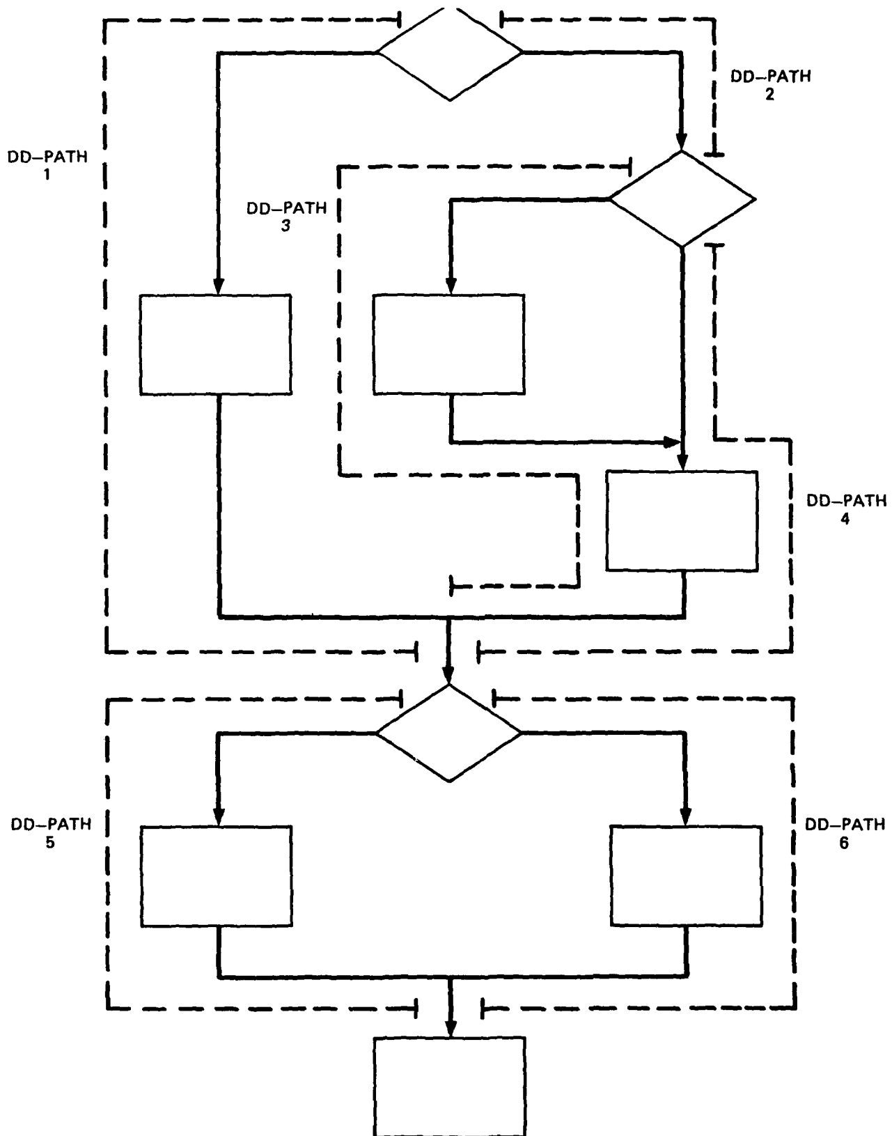
Figure 3-8. Sample Application Flowchart and Test Paths
