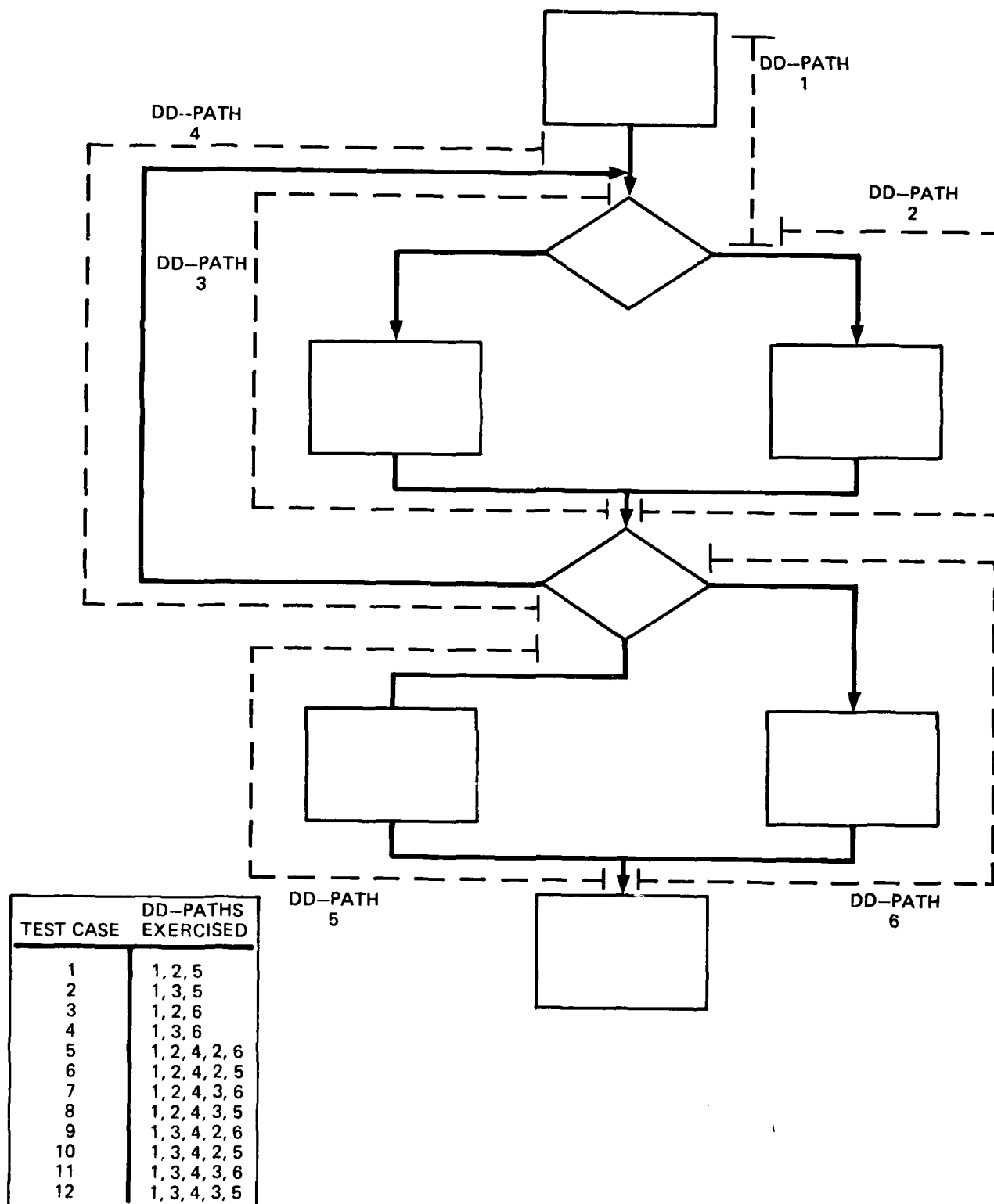
Figure 3-3. Flow Diagram With Test Cases
