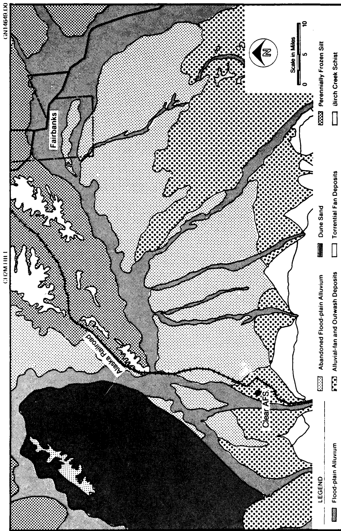
FIGURE 5. Geologic map.
