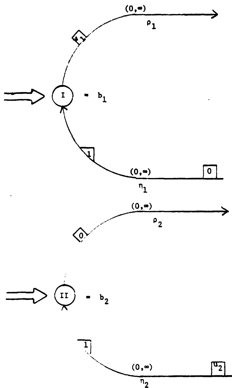
Figure 6-1: g_t(\bar{n}, \bar{\rho}) = w_1 \rho_1 + u_2 \eta_2
