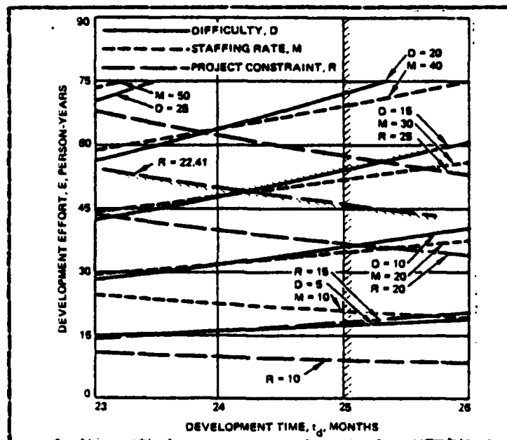
Figure 2.4 Feasible Solution Region
