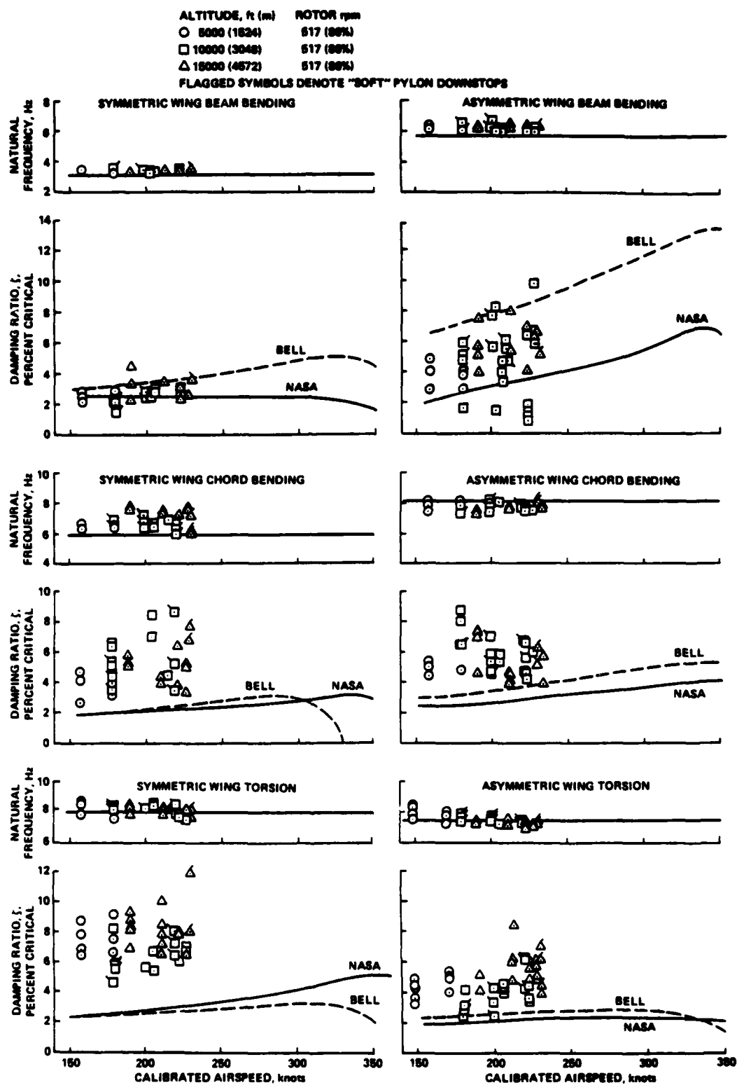
Fig. 13. Summary of aeroelastic stability data.
