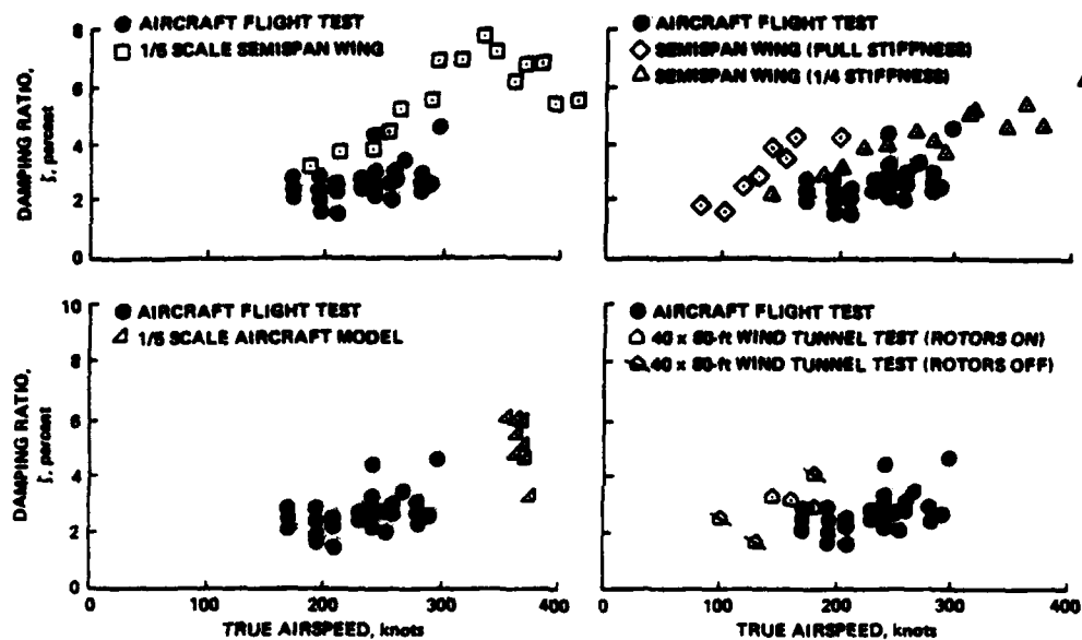
Fig. 16. Test data from 4 major tests.
