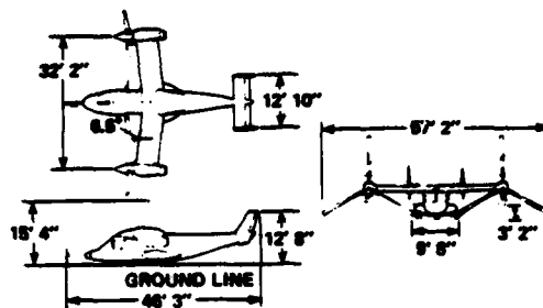
Fig. 7. XV-15 dimensions.
