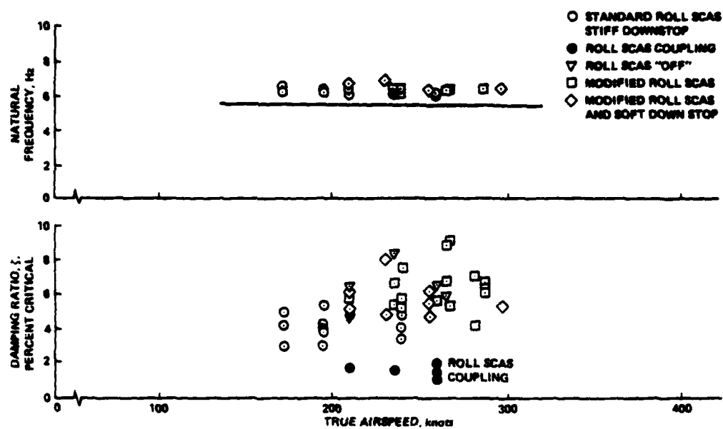
Fig. 14. Roll SCAS coupling.
