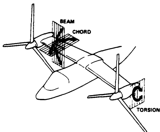
Fig. 8. XV-15 rotor/pylon/wing aeroelastic modes.
