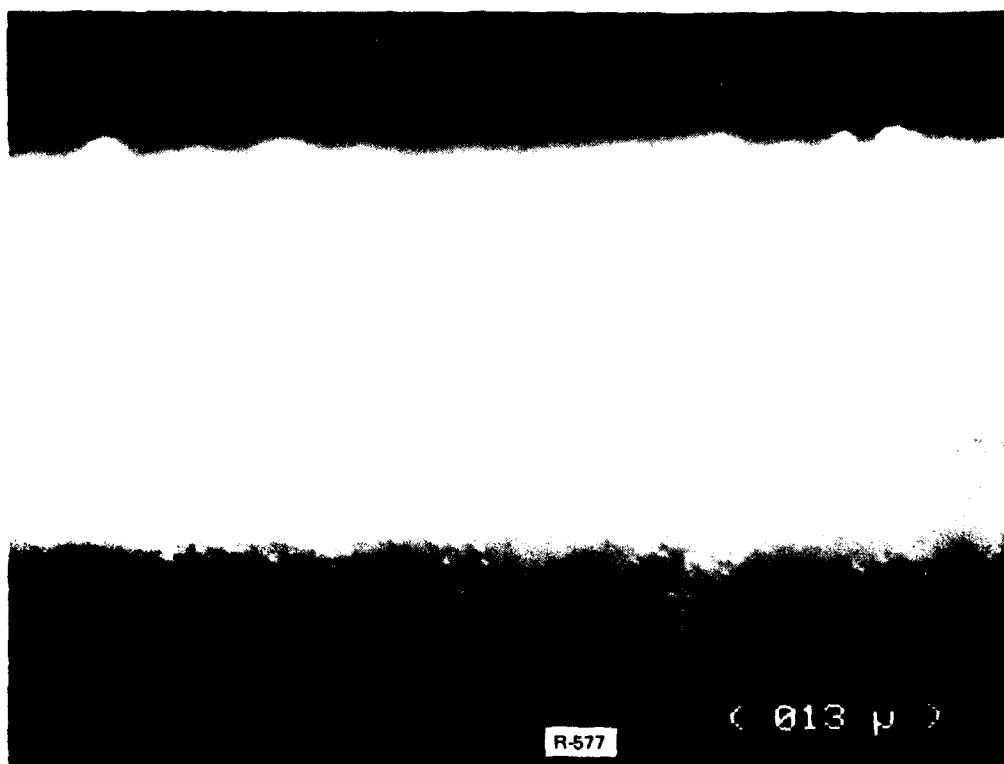
Fig. 2 Electron micrograph of tantalum carbide coating; upper picture--top view; lower picture--cross section. Tungsten carbide coatings appear similar.
