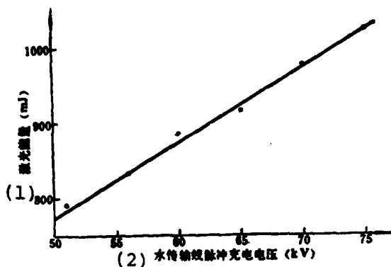
Fig. 4 The XeCl*3080Å Laser Output Energy Changes With the Water Transmission Line's Pulse Charging Voltage
