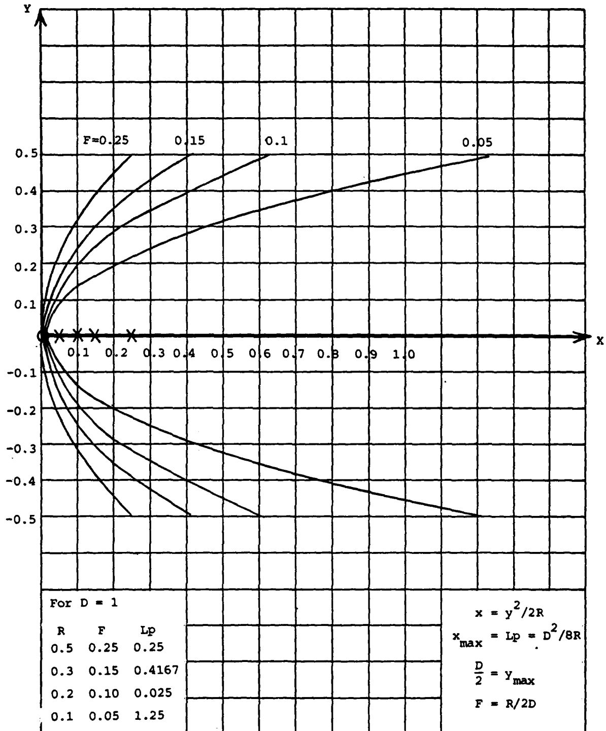
Fig. 4.4 Paraboids of various F/number and fixed aperture.
