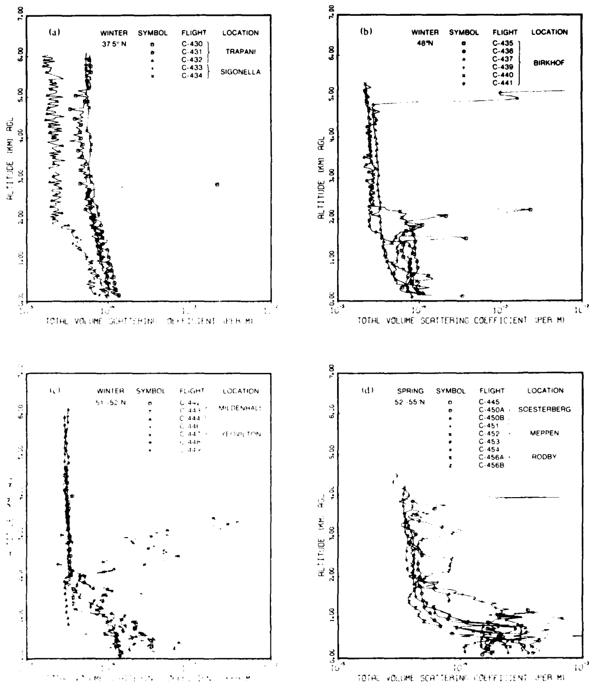
Fig. 2.3. Total volume scattering coefficient for filter 4 pseudo-photopics for OPAQUE IV flights 31 January through 31 March 1978 (AFGL-TR-79-6159)
