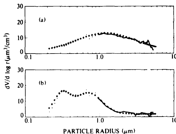
Fig. 3-3. The volume distribution sampled at Yeovil (a) and at Rodby (b) during March at an altitude of 152m. The fit of Eq. (1) to the data (+) is shown for comparison.
