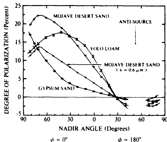
FIG. 5. Degree of polarization of radiation reflected from gypsum sand, Mojave Desert sand and Yolo loam in the principal plane for \lambda = 0.4 \mu\text{m} and \theta_0 = 53^\circ , and for Mojave Desert sand for \lambda = 0.6 \mu\text{m} and \theta_0 = 53^\circ .
