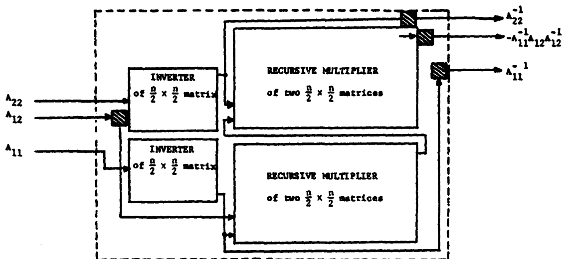
Figure 1. Layout of the recursive matrix inverter; Shaded boxes are data buffers.
