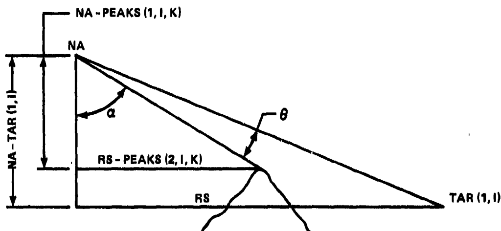
Figure B-3. Variables Used to Calculate a Peak Clearance Equal to at Least the Laser System Buffer Zone
