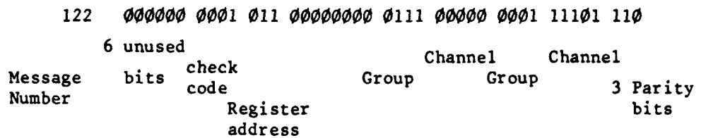
FIGURE 8 - MESSAGE WITH SEGMENTATION 3 (MATRIX CONNECTION )
