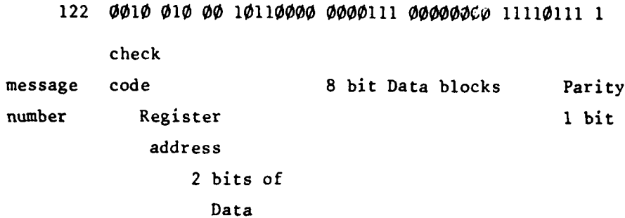
FIGURE 6 - MESSAGE WITH SEGMENTATION 1
