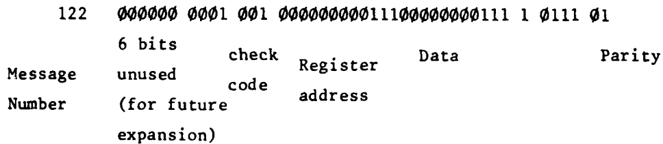
FIGURE 7 - MESSAGE WITH SEGMENTATION 2 (MATRIX STATUS)
