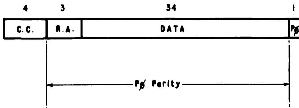
FIGURE 1 - GTU MESSAGE FORMAT
