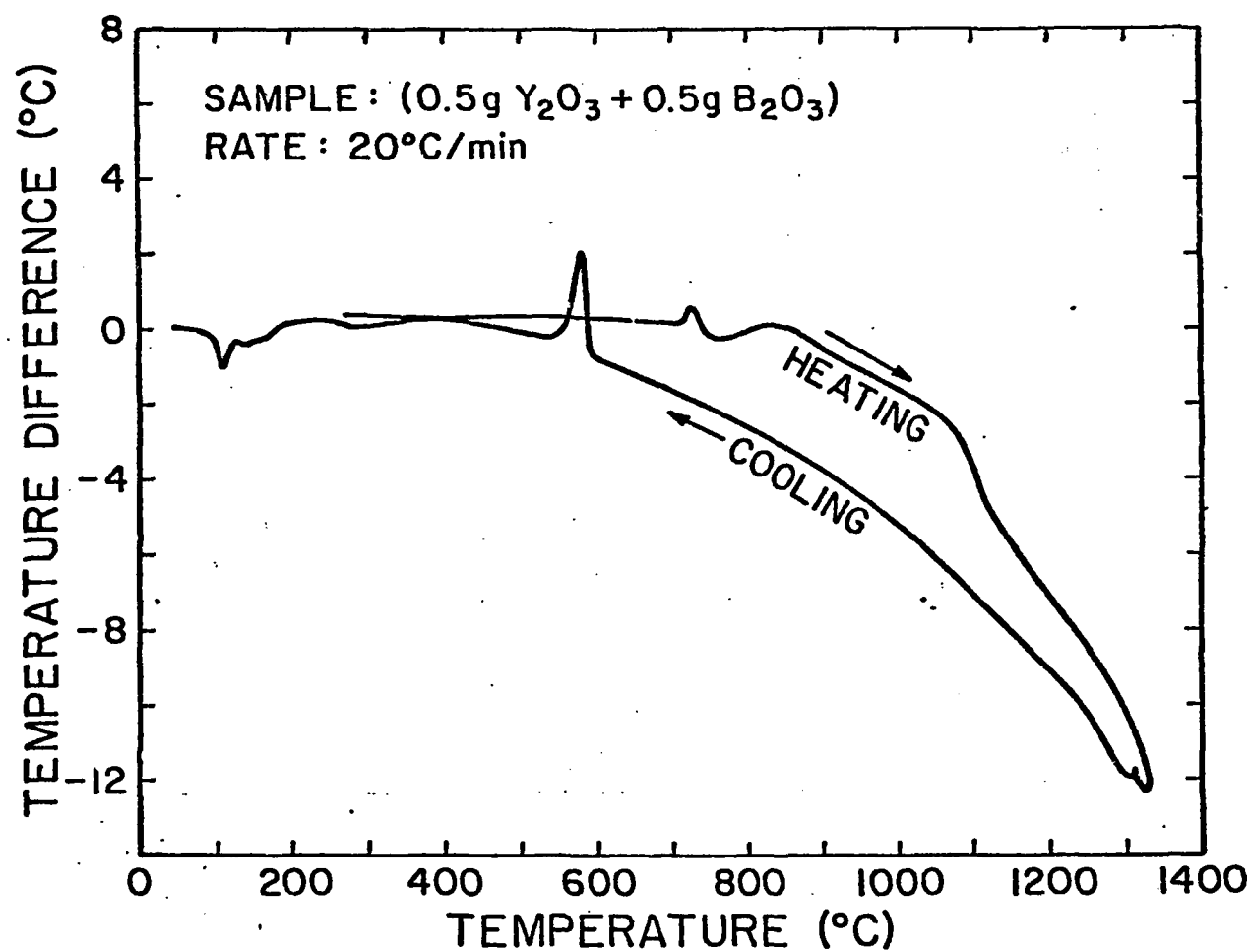
Fig. 1. DTA traces for (1:1) \text{Y}_2\text{O}_3\text{:B}_2\text{O}_3 sample showing heating reactions and phase formation ( \sim 600^\circ\text{C} ) on cooling.
