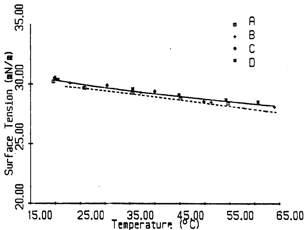
Figure 17 Variation of the Surface Tension with Temperature for Tmp-Heptanoate Containing Tricresyl Phosphate. Broken Line is Solvent Alone; A is 2.05% (w/w) Tricresyl Phosphate; B is 1.99% (w/w) Tricresyl Phosphate; C is 1.99% (w/w) Tricresyl Phosphate; D is 1.99% (w/w) Tricresyl Phosphate, Temperature increasing.
