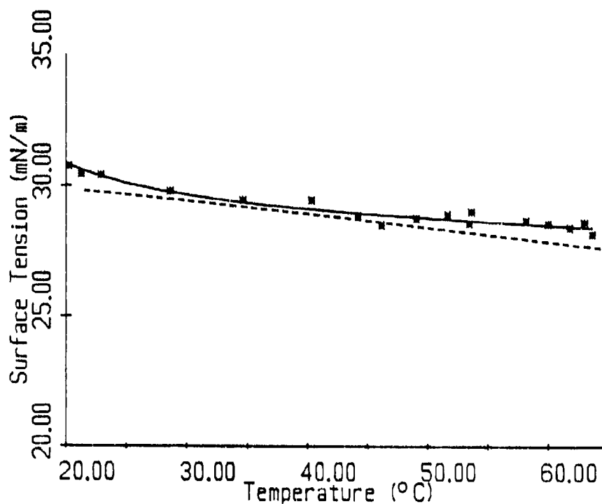
Figure 16 Variation of the Surface Tension with Temperature for Tmp-Heptanoate Containing Quinizarin Broken Line is Solvent Alone; Continuous Line is 0.0477% (w/w) Quinizarin
