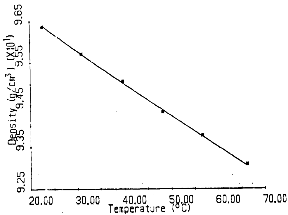
Figure 11 Variation of Density with Temperature for Tmp-Heptanoate Containing Phenothiazine (1.86% w/w)
