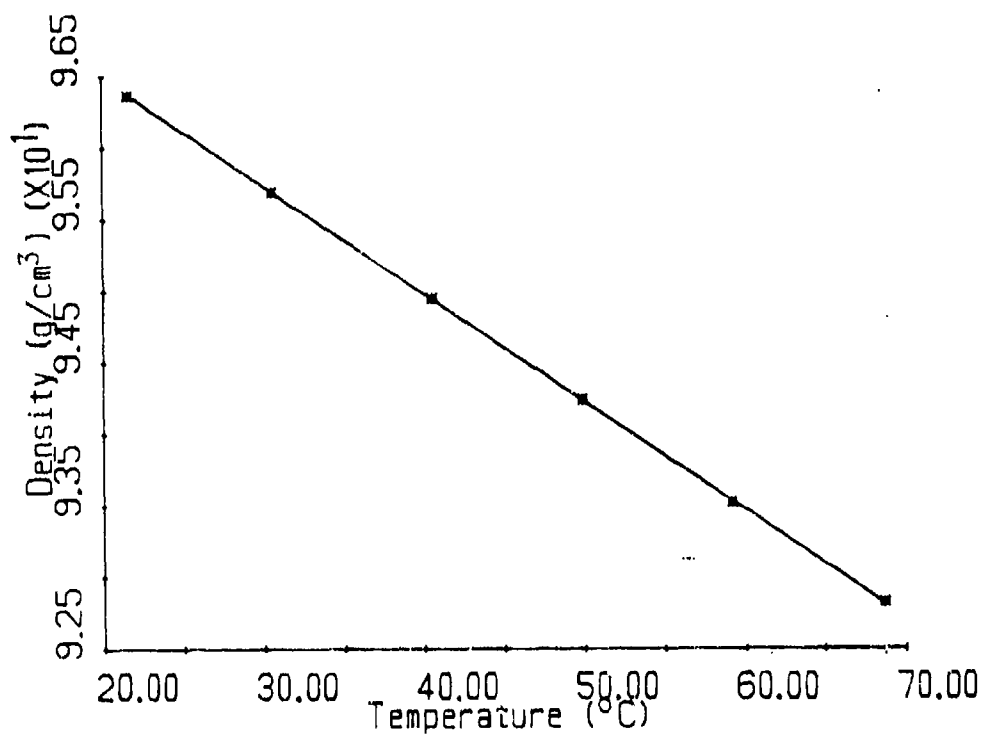
Figure 12 Variation of Density with Temperature for Tmp-Heptanoate Containing Tricresyl Phosphate (2.05% w/w)
