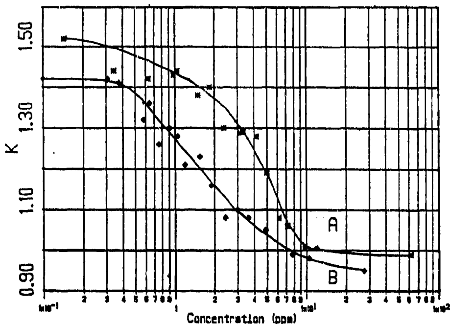
Figure 26 Comparative Rate of Ascension of Air Bubbles in Oils containing Polydimethylsiloxane (1000 cSt), T = 22^{\circ}\text{C} . Values of K are Corrected for the Wall Effect. A is Mineral Oil; B is Tmp-Heptanoate.
