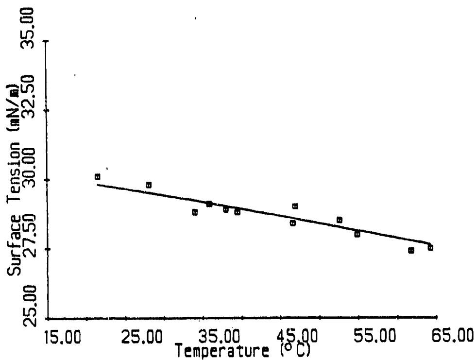
Figure 2 Variation of Surface Tension with Temperature for Tmp-Heptanoate
