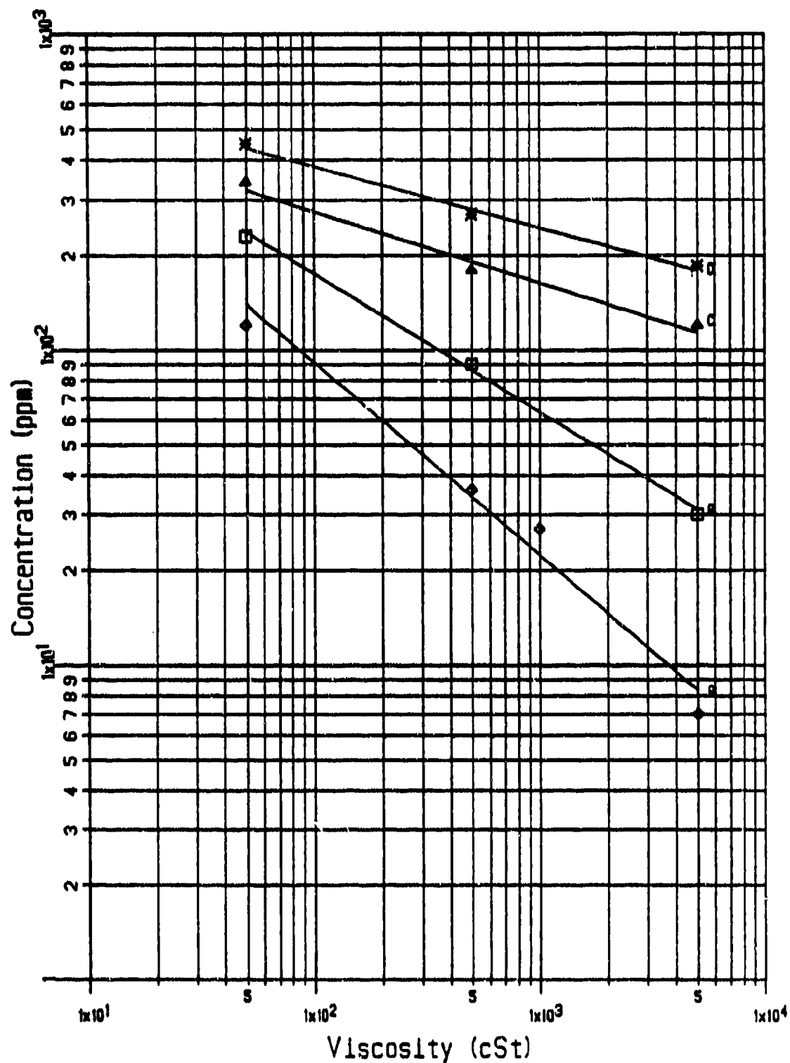
Figure 4 Variation of Solubility of Polydimethylsiloxane in Various Solvents at 20°C as a Function of its Kinematic Viscosity. Solvents are: A = Timp-Heptanoate; B = Timp-Heptanoate containing 10% Toluene (v/v); C = Timp-Heptanoate containing 20% Toluene (v/v); D = Timp-Heptanoate containing 30% Toluene (v/v)
