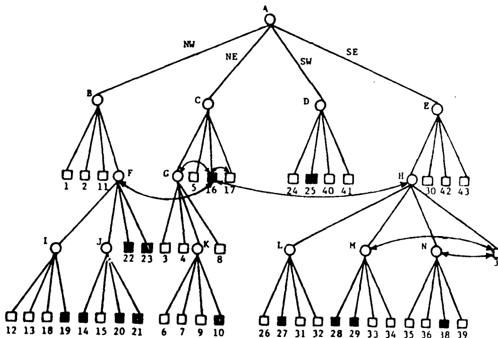
Figure 2.1. A region, its maximal blocks, and the corresponding quadtree. Blocks in the region are shaded, background blocks are blank. Horizontal lines indicate ropes.
