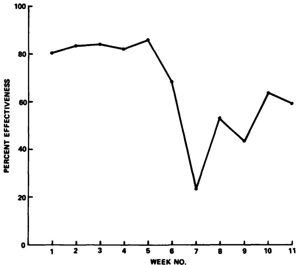
Figure 9. Percent effectiveness of operational fragment barrier, Okanogan River, Oroville, Wash., during the period 29 July-13 October 1979, based on wet weight of material collected on upstream (No. 1) and downstream (No. 2) evaluation barriers
