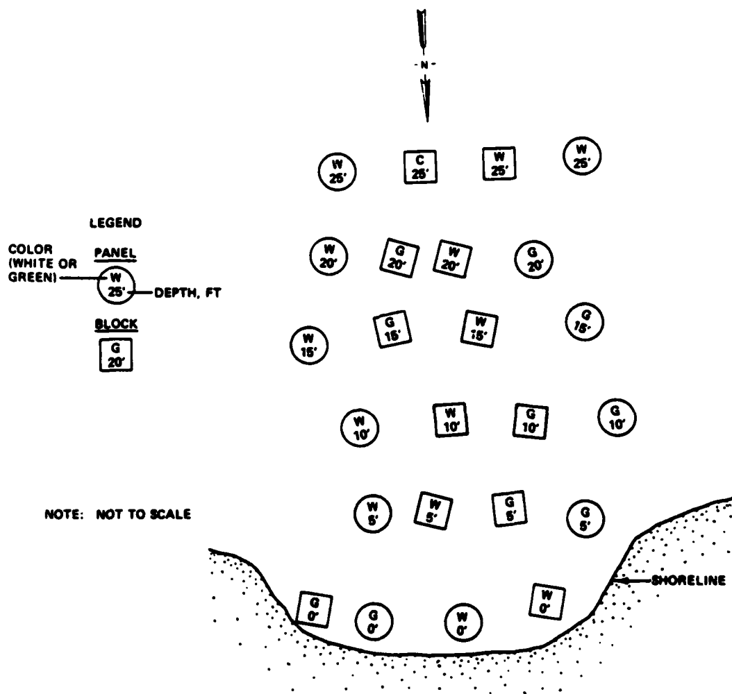
Figure 2. Layout of underwater target panels and blocks used at Lake Whatcom
