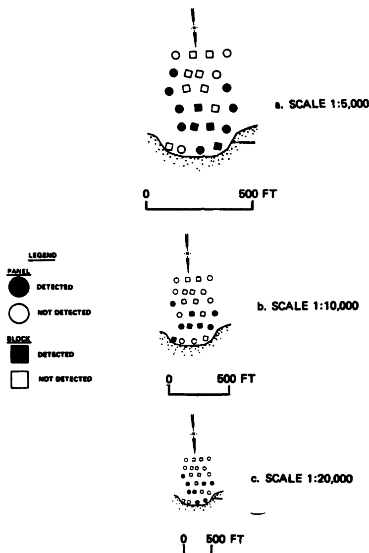
Figure 3. Underwater target panels and blocks detected on three scales of color imagery, Lake Whatcom
