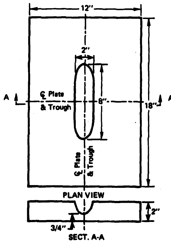
Figure 6-13 DTNSRDC tough Weldability specimen.
