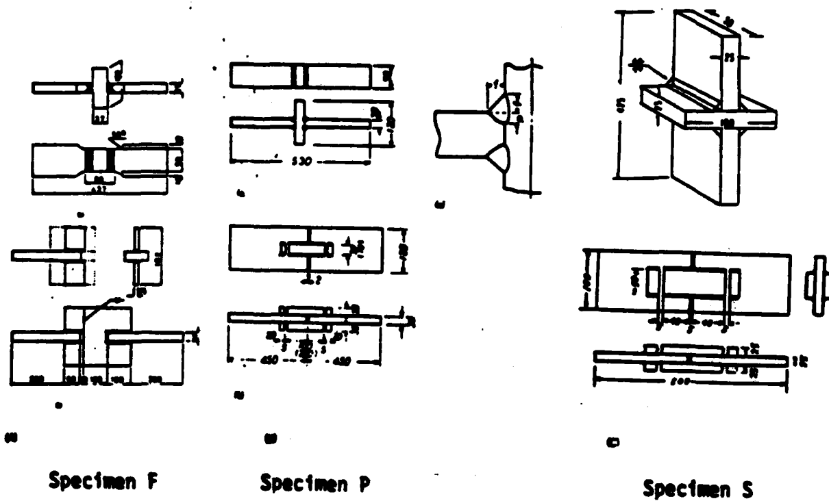
Figure C-23 Specimen geometry.
