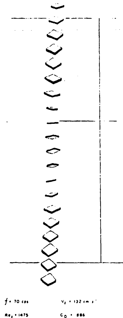
Figure 10. Stroboscopic Picture of a Quietly Settling Paper Square (1.4 x 1.4 cm 2 ).
