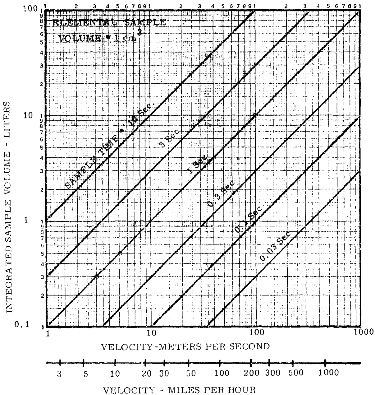
Figure 4.1. Integrated sample volume vs air speed for an elemental scattering volume of 1 \text{ cm}^3 at six different sample times.
