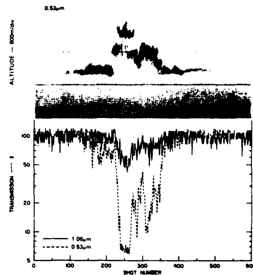
Fig. 3. Cross-plume structure derived from ALPHA-1 plume backscatter and vertical transmissions derived from surface returns at 1.06\text{-} and 0.53\text{-}\mu\text{m} wavelengths (aircraft pass 2).
