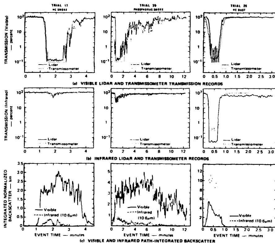
Fig. 5. Comparison of transmissions derived from lidar target returns and transmissometer records for (a) visible, (b) infrared systems, and (c) path-integrated backscatter for three Smoke Week II trials.
