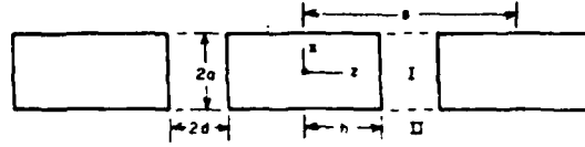
Fig. 2 Periodic collinear array of cylinders
