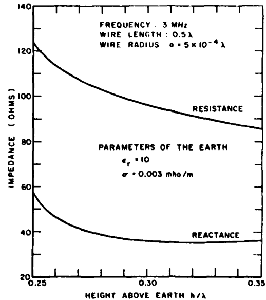
Fig. 1. Impedance of center-fed vertical wire versus height above the earth.
