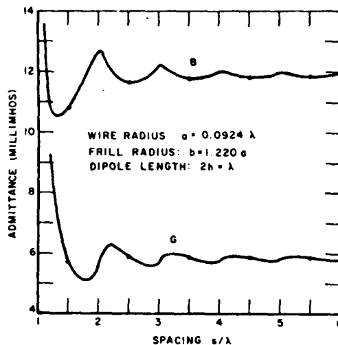
Fig. 6. Admittance versus spacing for periodic collinear array of solid center-fed cylindrical antennas with flat ends.
