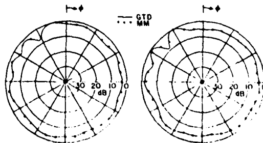
Fig. 20. GTD-MM comparison with electric line source using geometry shown in Figure 19 with L = 2.0\lambda , D = 0.05\lambda , \epsilon_r = 2.0 (Left) \phi_o = 20^\circ and (right) \phi_o = 40^\circ .
