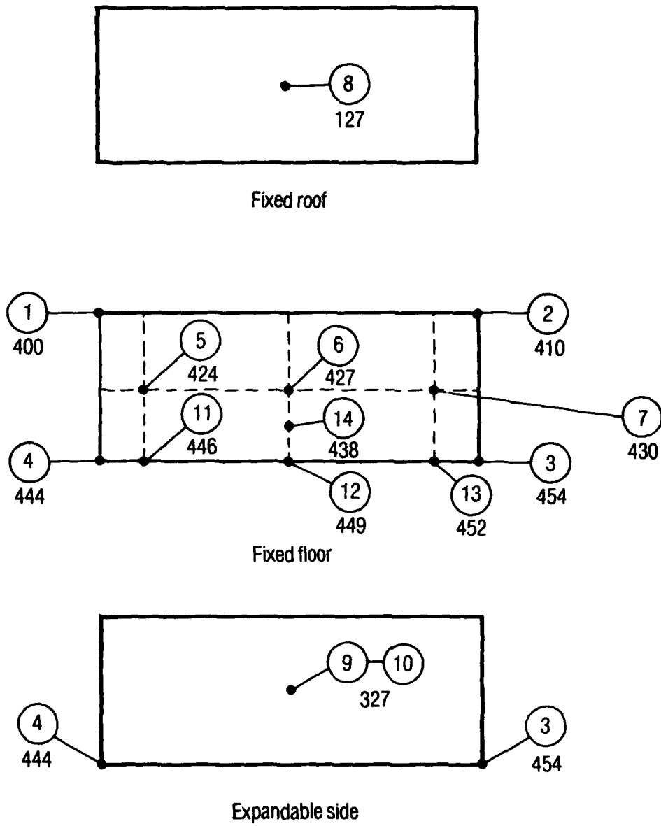
Figure 25. Location of points where accelerations were measured for the end drop test.
