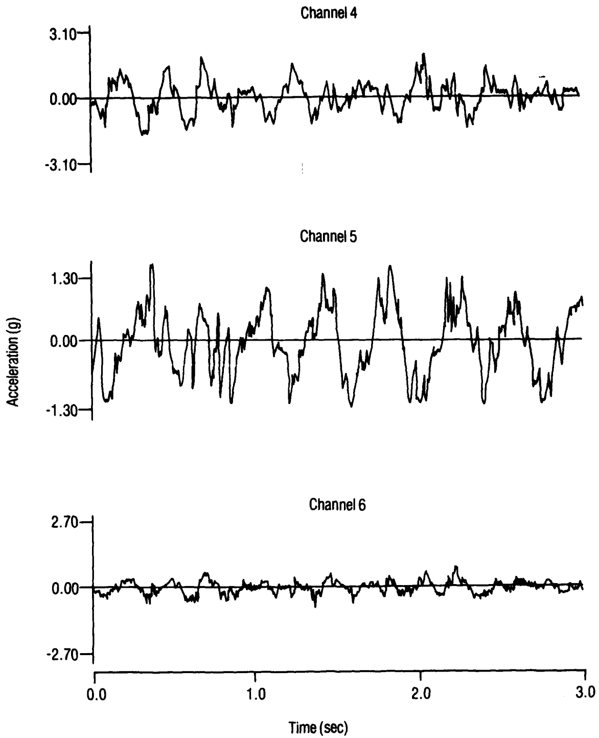
Figure 31. Contiued. Acceleration vs time, Belgian block test, channels 4, 5, and 6.
