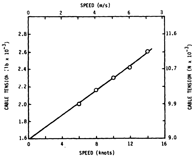
Figure 3b - Cable Tension at the Depressor
