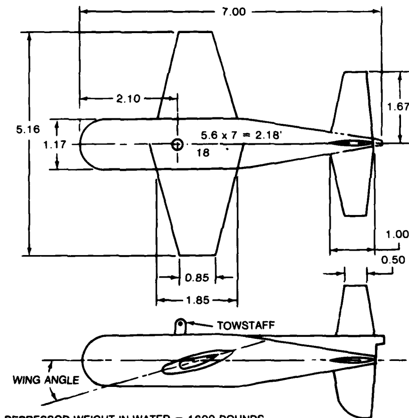
Figure 1 - DTNSRDC Depressor
