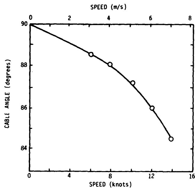
Figure 3a - Cable Angle at the Depressor
