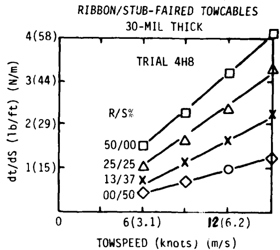
Figure A.1 - Towcable Tension per Unit Length versus Towspeed for Various Towcables
