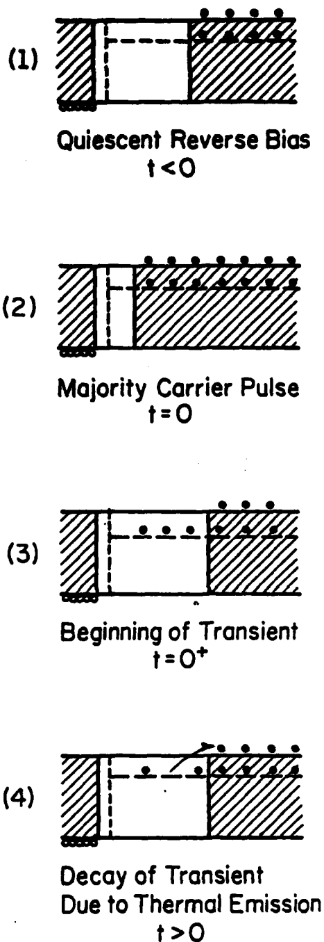
Fig. 2.5. Capacitance transient due to a majority carrier trap in a p^+-n diode. The insets labeled 1 through 4 schematically show the charge state of the defect level and width of the space charge region (unshaded portion) at various times before and during the transient [14].
