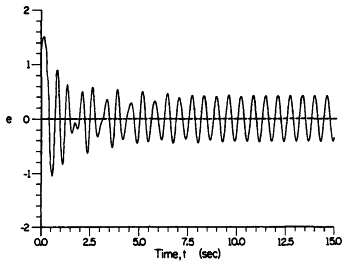
Fig. 5.9 Tracking results for \mu = 0.05 , e(0) = 1 , \eta(0) = 1 , K(0) = 3 , \sigma = 0.08 and r(t) = 3\sin 10t .
