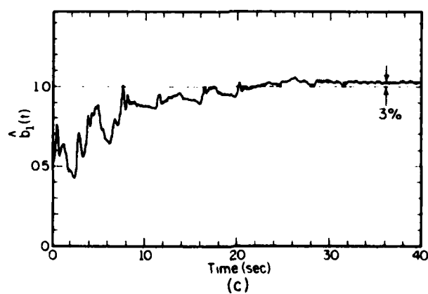
Fig. 2.3 Identification results for \mu = 0.05 and u = 5\sin t + 5\sin 2.5t ( \gamma = 18.2 ).
