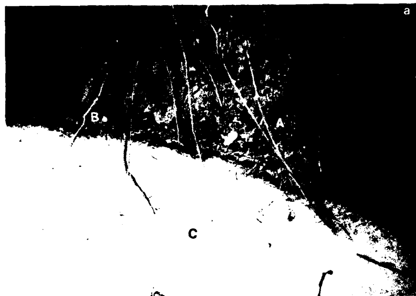
a. Bank sediment (A) sloughing (B) onto nearshore ice (C) (15 December 1981).
