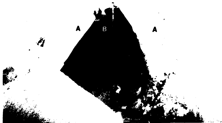
Figure 16. Ice (A) and shore sediment (B) uplifted (about 60 cm) where an ice pressure ridge intersects the shoreline (30 January 1980, Orwell Reservoir, Minnesota).
