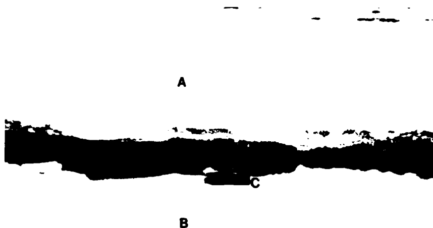
a. The shelf (A) is below the bank toe (B) and is separated from and higher than the ice cover (C), which is being lowered as the water level drops.
