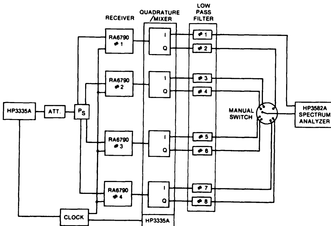
Figure 1. Measurement Equipment Configuration
