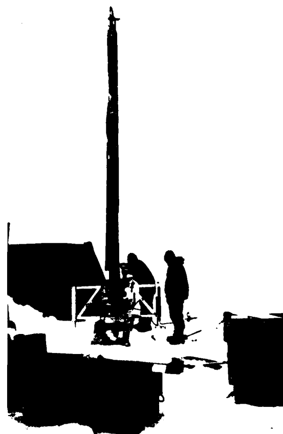
Figure 5. Electromechanical drill hoist assembly used for coring into the ice shelf.
