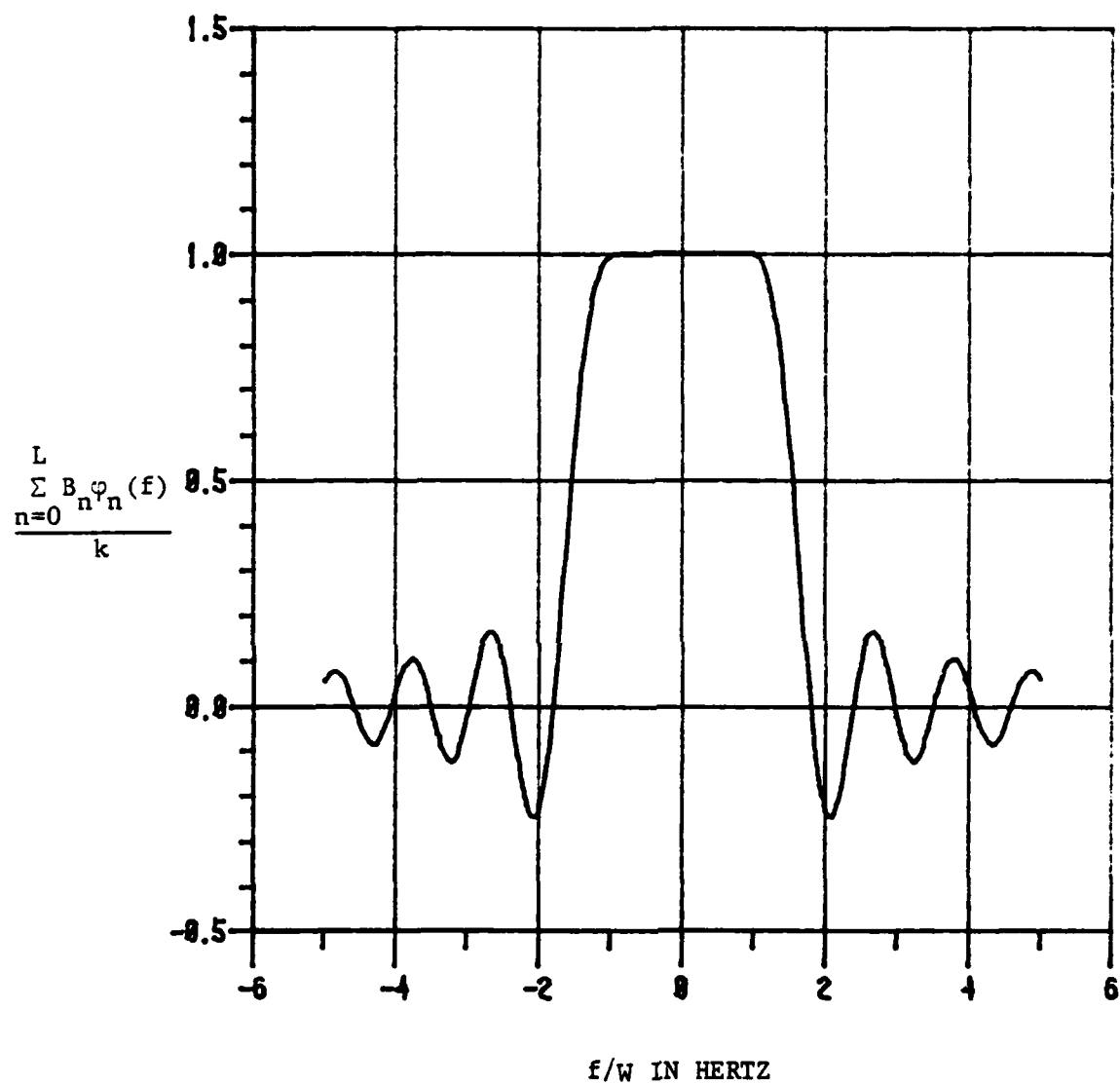
Figure 4.1. \frac{L}{k} \sum_{n=0}^L B_n \varphi_n(f) vs. f/W, (W = \frac{6}{\pi T_c}, L = 8)
