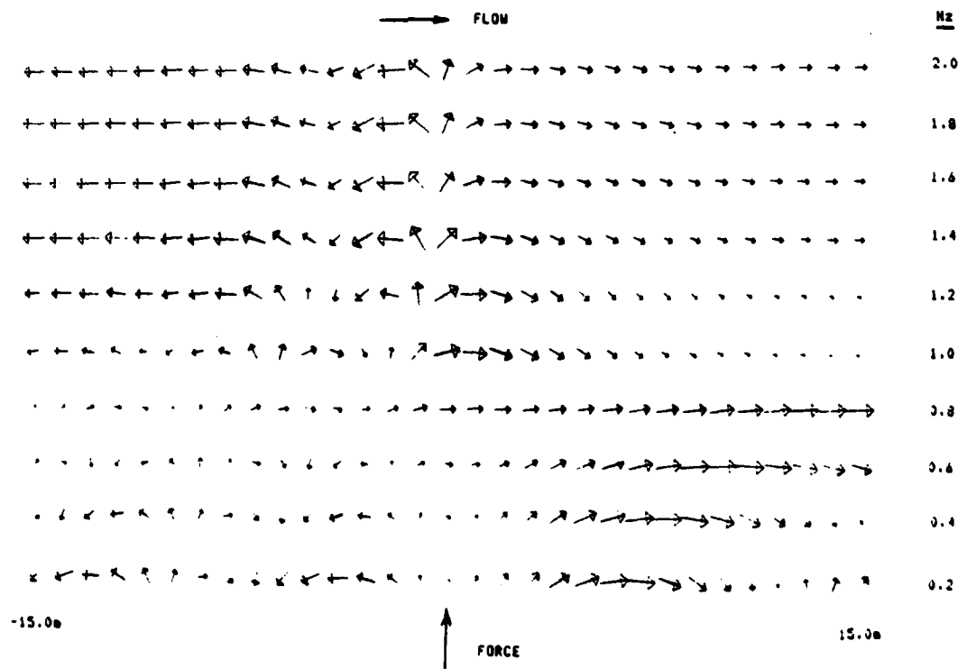
FIG. 15 INTENSITY VECTORS ALONG PLATE SURFACE U=22.5m/s, FORMULATION 1
