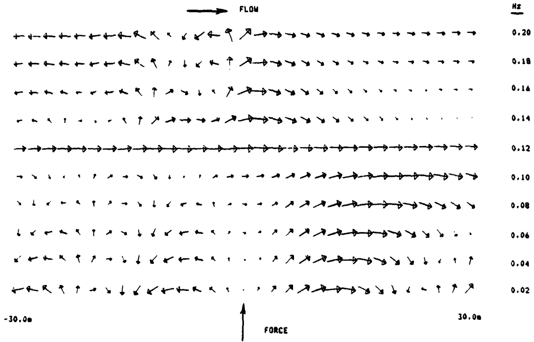
FIG. 12 INTENSITY VECTORS ALONG PLATE SURFACE U=7.5m/s, FORMULATION 1
