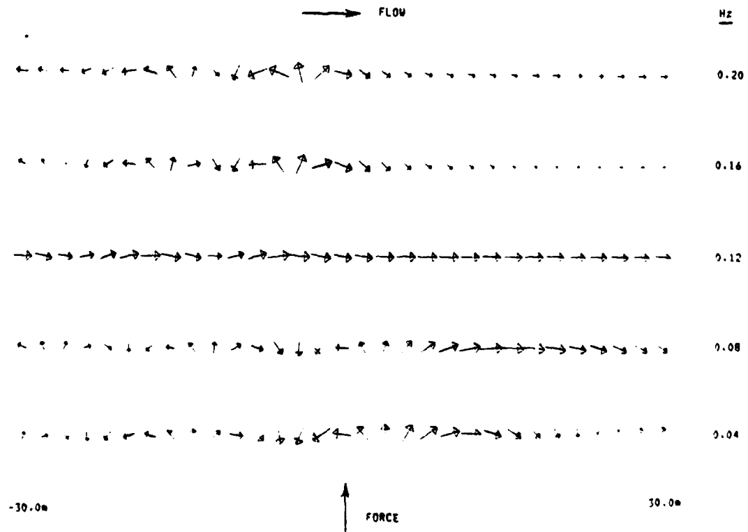
FIG. 13 INTENSITY VECTORS ALONG PLATE SURFACE U=7.5m/s, FORMULATION 2
