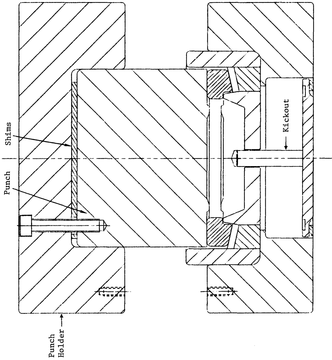
FIGURE 13. Schematic of the Forging Tooling
