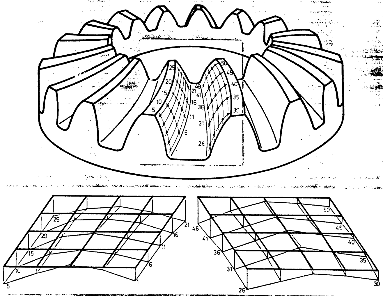
FIGURE C-14. Three-Dimensional Representation of Gear Tooth Profile Measurements
