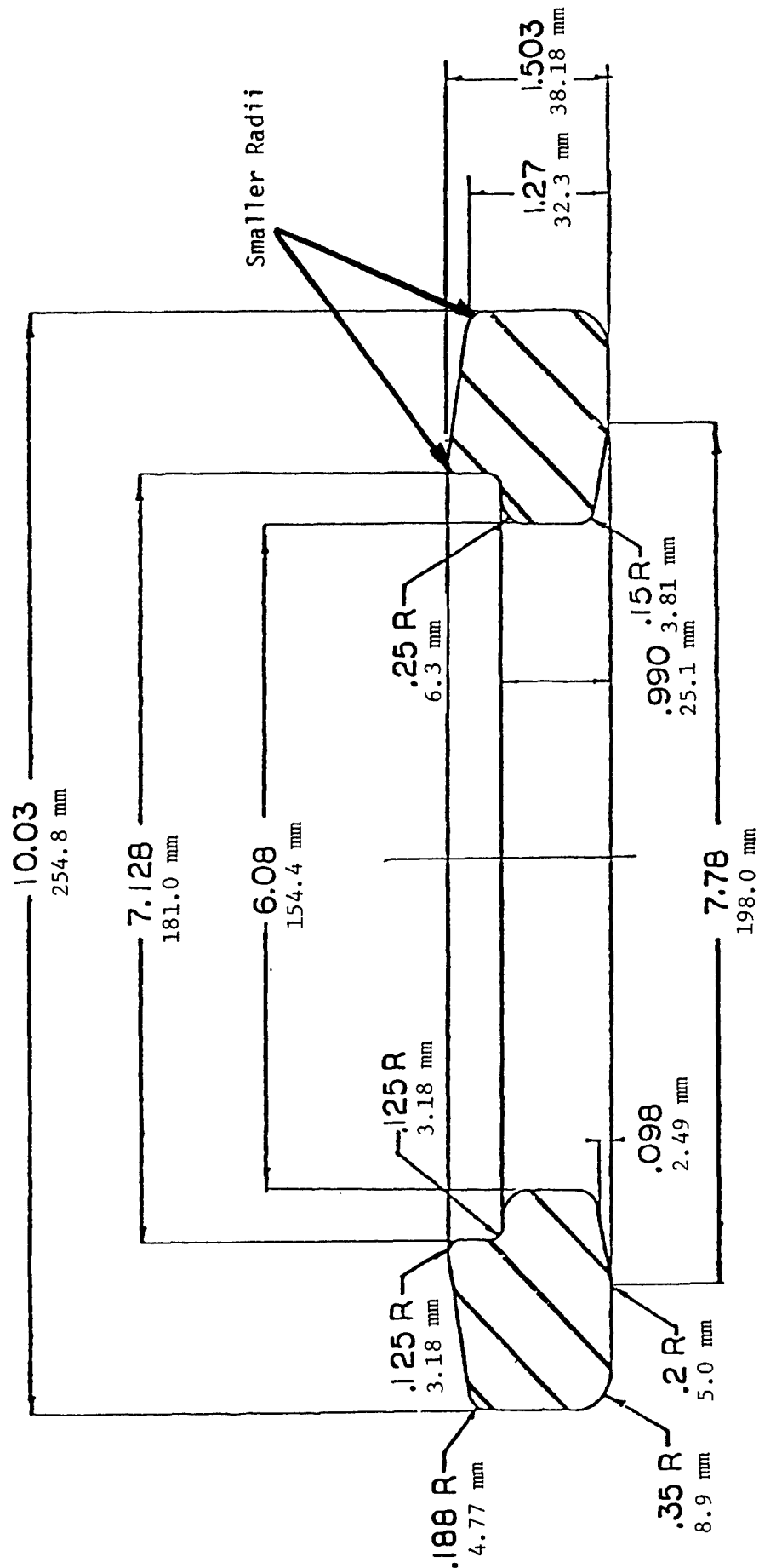
FIGURE B-9. Preform Design (Type B) Used in Net Forging Trials (Third Series) (Preform material: 8620 steel)
