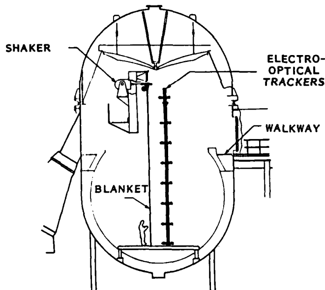
TEST ARRANGEMENT
