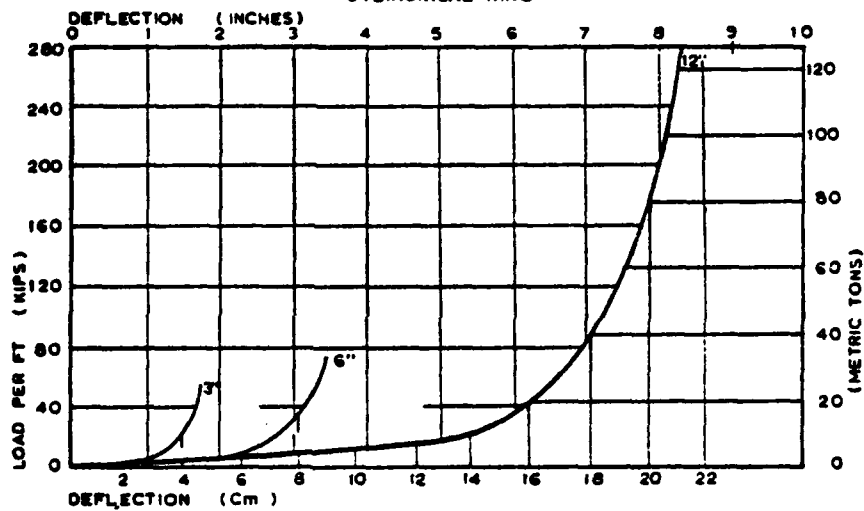
APPROXIMATE LOAD/ ENERGY, DEFLECTION CURVES FOR MORSE STANDARD CYLINDRICAL WING
