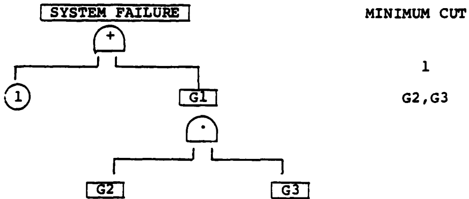
Figure 3.3. Second Level of the Fault Tree
