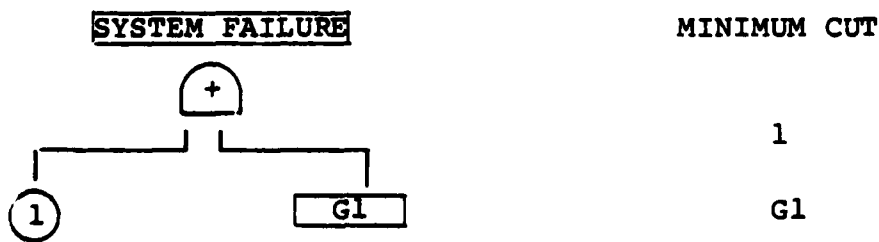
Figure 3.2. First Level of the Fault Tree
