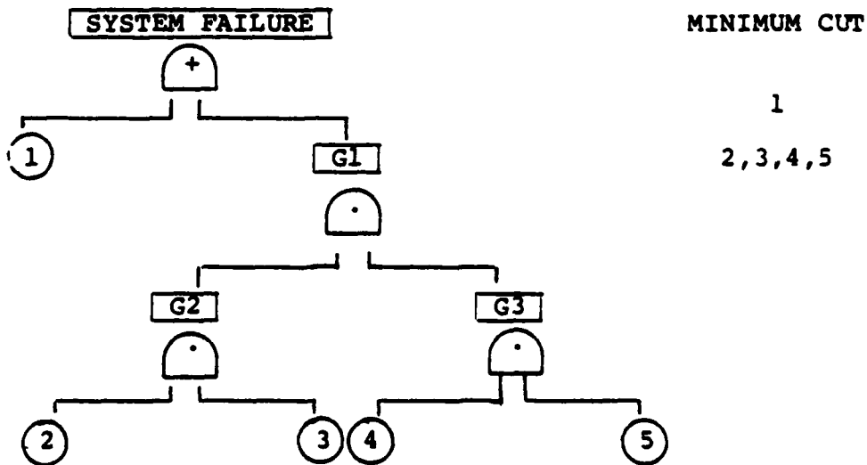
Figure 3.4. The Complete Fault Tree and Its Minimum Cut Representation
