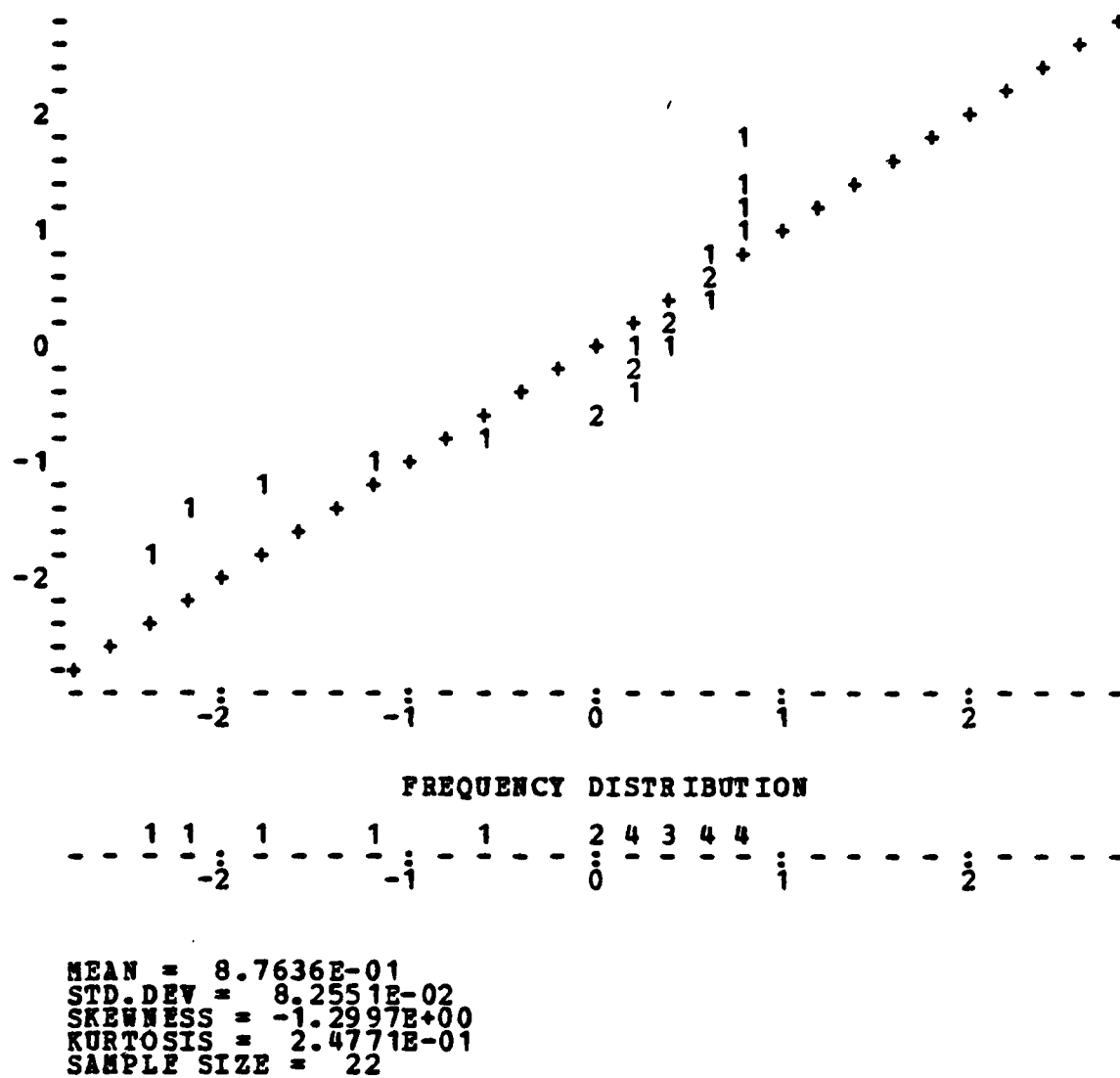
Figure 3. Normal Probability Plot of the Variable PE
