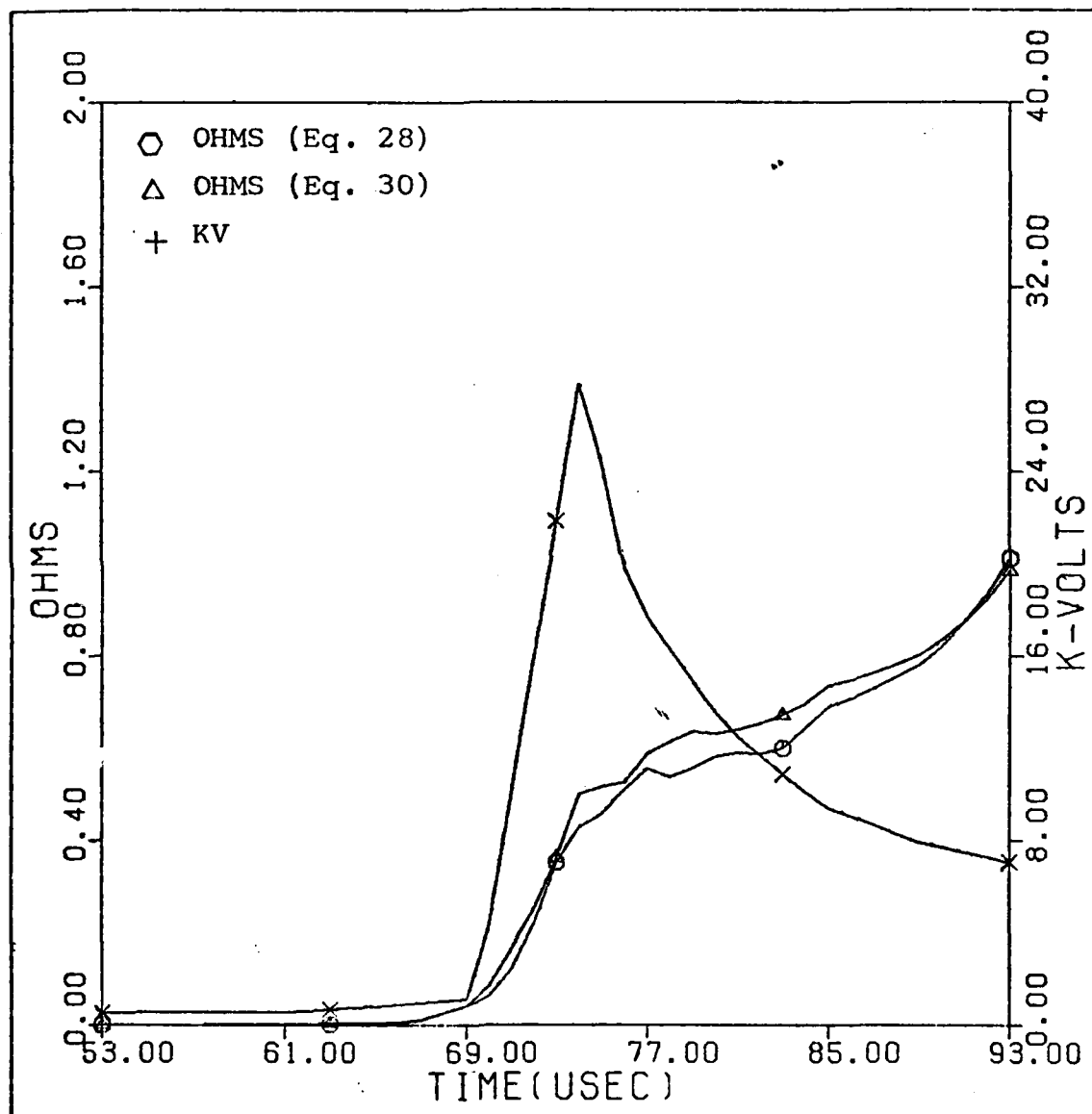
Fig. 49 Switch P8 Resistance and Voltage
