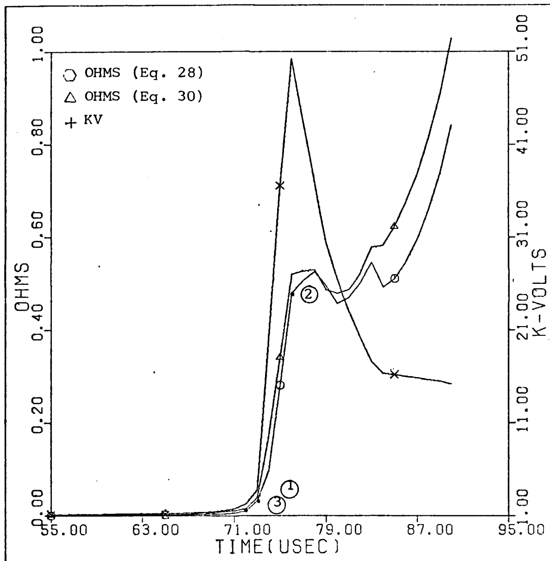
Fig. 17 Plot of Switch P10 Resistance and Voltage
