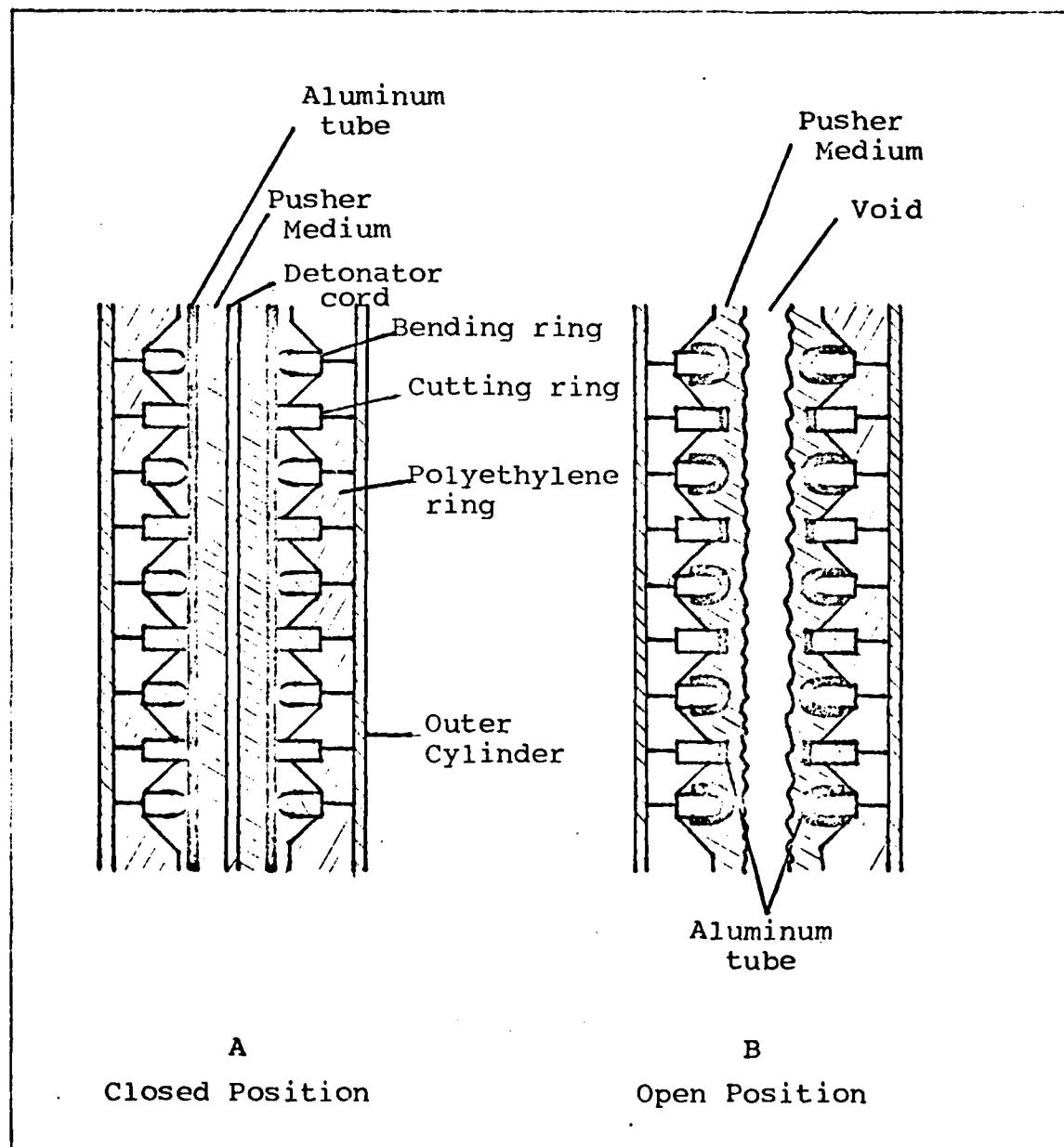
Fig. 6 Cross Section of Cylindrical Switch in the Open and Closed States.
