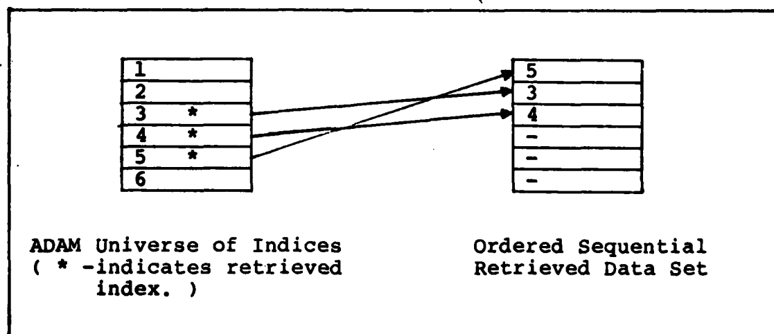
Fig 9. ADAM Ordered Sequential Retrieval
