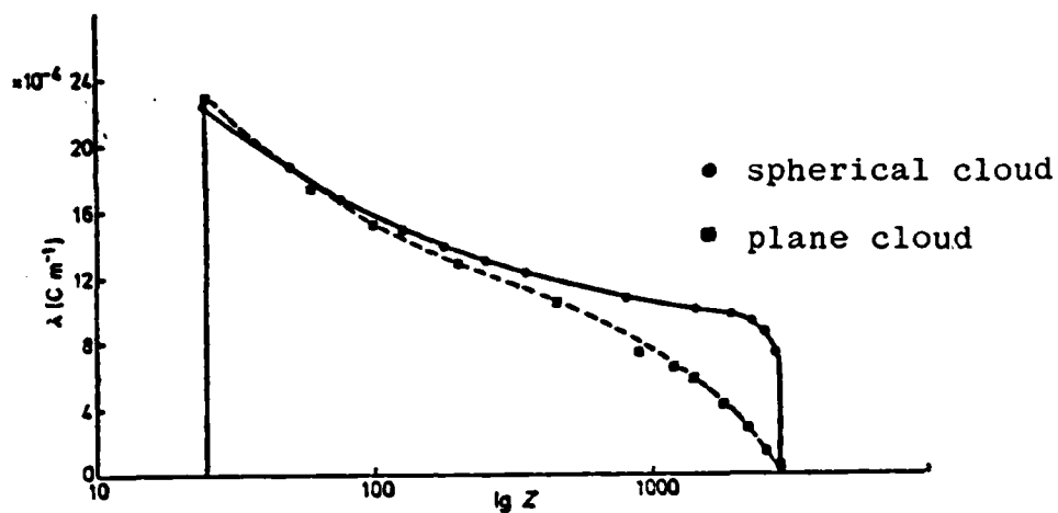
Fig 4.4a Distribution of Linear Charge Density \lambda Along 3 km Lightning Channel for Two Clouds Model (Little, 1978).
