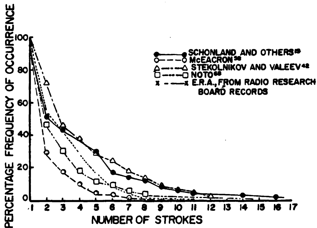
Fig 2.2 Number of Successive Strokes in Lightning Flashes (Adapted from Bruce & Golde, 1941).
