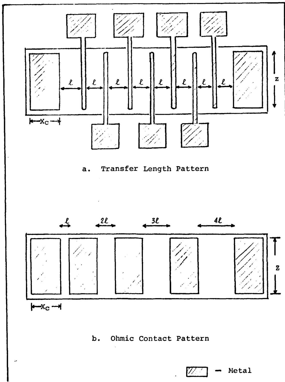
Figure 5. Test Pattern used to evaluate Specific Contact Resistivity
