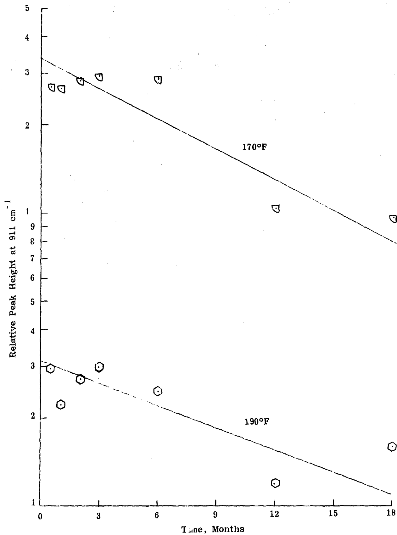
Figure 63. Variation in 911 cm -1 Peak Height with Age Time at 170° and 190°F (MSL-303 Propellant)
