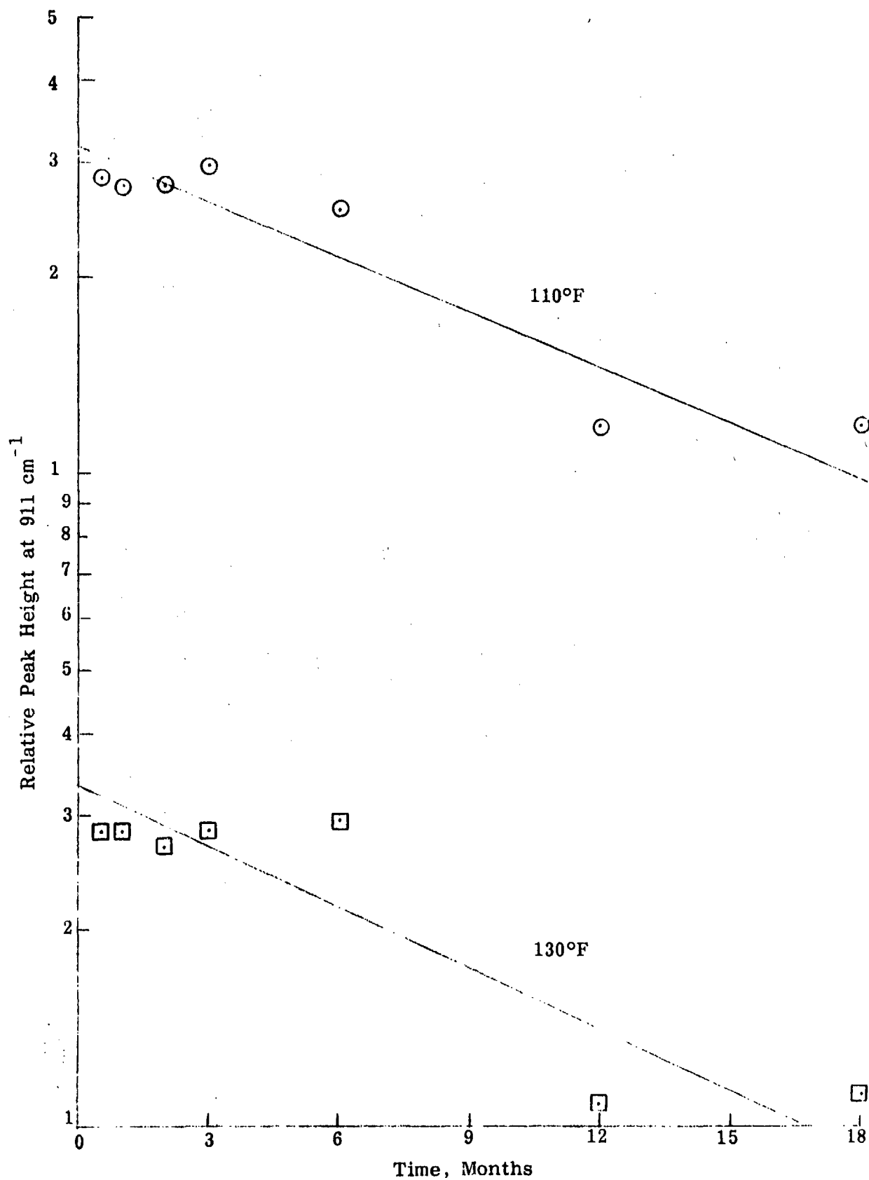
Figure 62. Variation in 911 cm -1 Peak Height with Age Time at 110° and 130°F. (MSL-303 Propellant)
