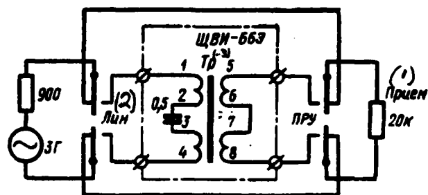
Fig. 7. KEY: (1) Reception. (2) Line. (3) Tr.
