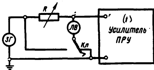
Fig. 5. ZG - audio generator; LV - tube voltmeter; R - Resistance box; Kl - key contact. KEY: (1) Amplifier.
