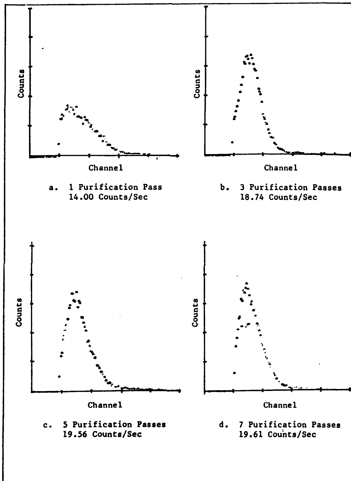
Figure 10. The Effects of Purification on the Spectrum of \text{Xe } 131\text{m}
