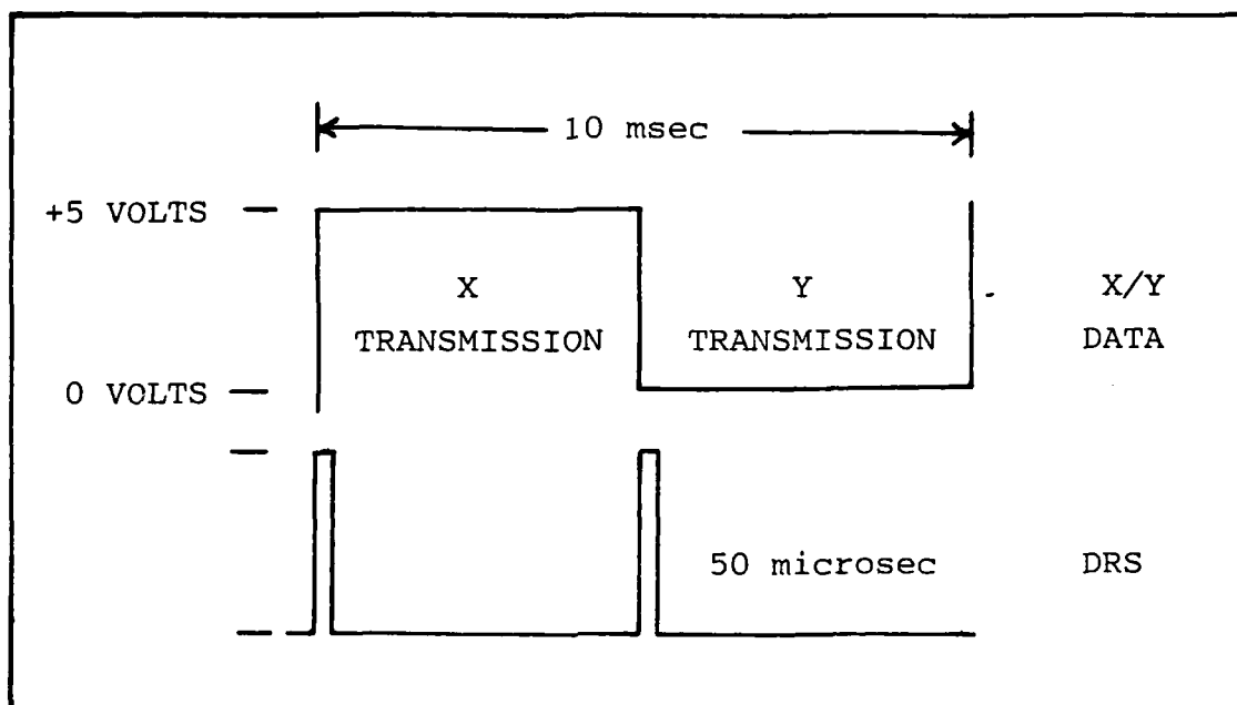
Fig. 6 Data Timing
