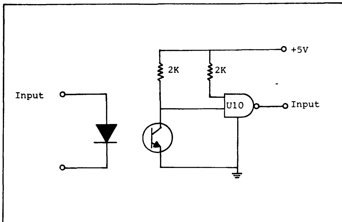
Fig. 19 Optoisolator Circuit (Ref 9 :139)
